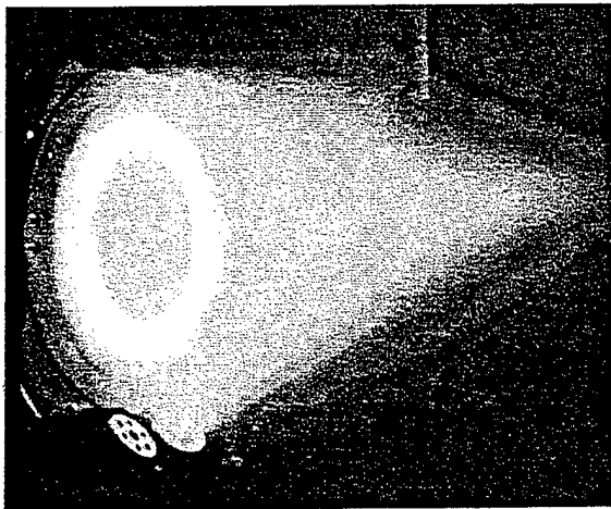
Fig. 1. Faked SPT-140 Demonstration Model 3 (DM3) firing in AFRL's long-duration test facility.
