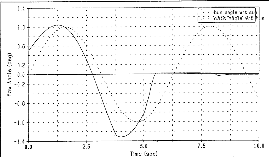
Figure 9. Concentrator and Engine Rotational Motion
