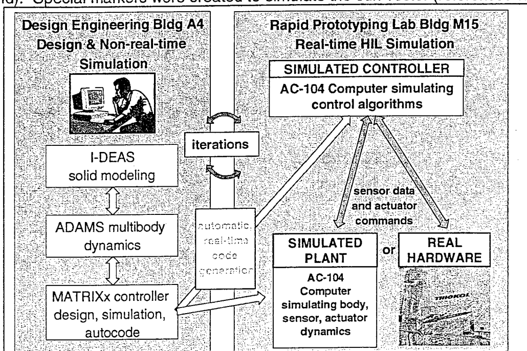
Figure 5. Rapid Prototyping Environment
