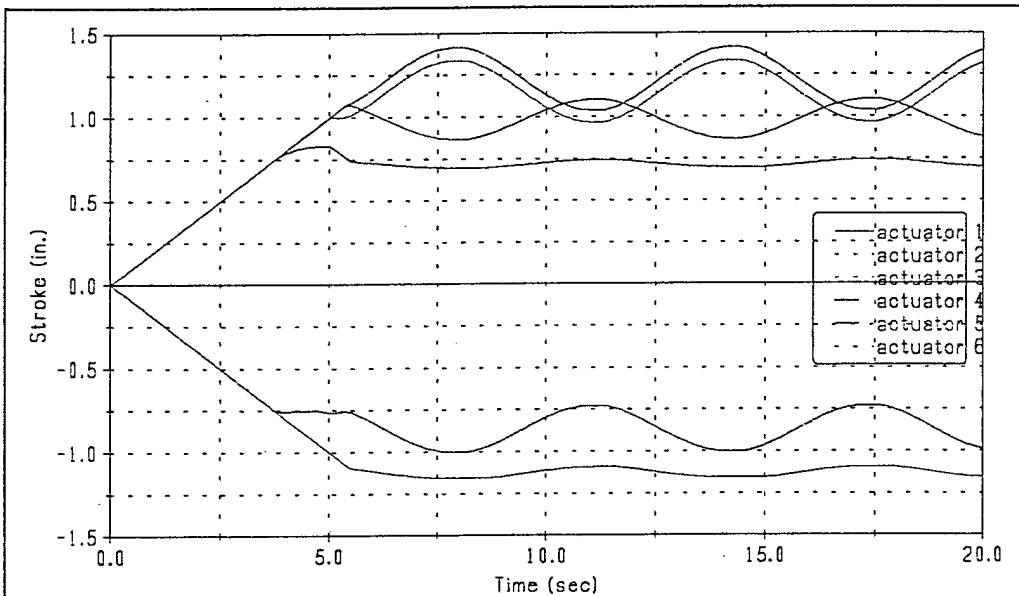
Figure 10. Linear Actuator Stroke
