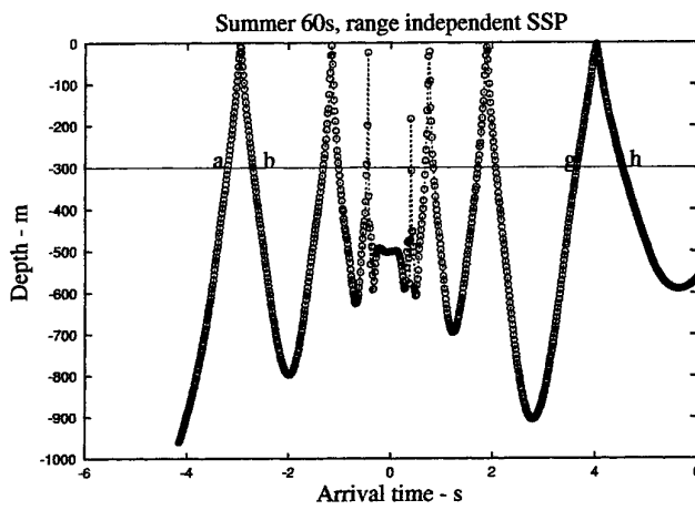
Figure 7: Ray fan summer 60, no range dependence
