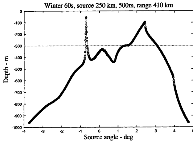
Figure 6: Ray fan winter 60, depth against source angle
