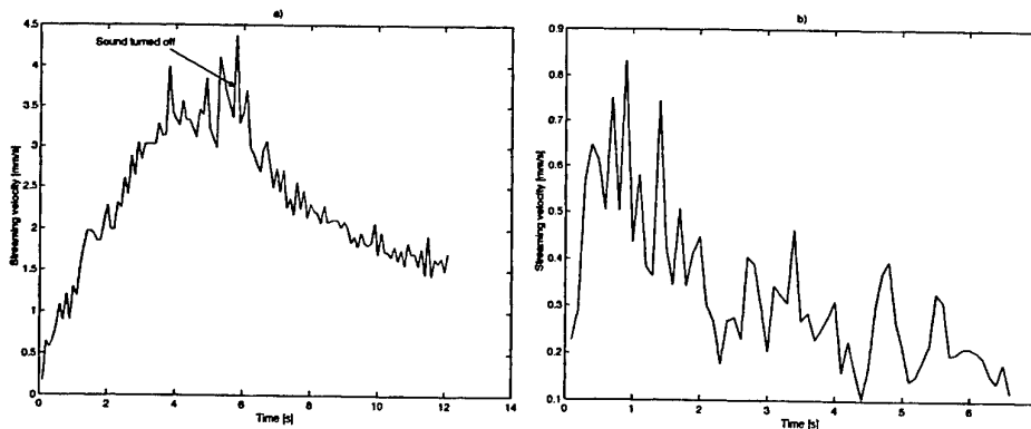
Figure 6: Acoustic streaming, decay and rise time. a) 10 Hz burst repetition frequency, b) single burst.
