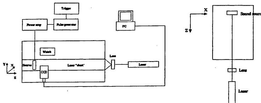
Figure 1: Experimental setup.
