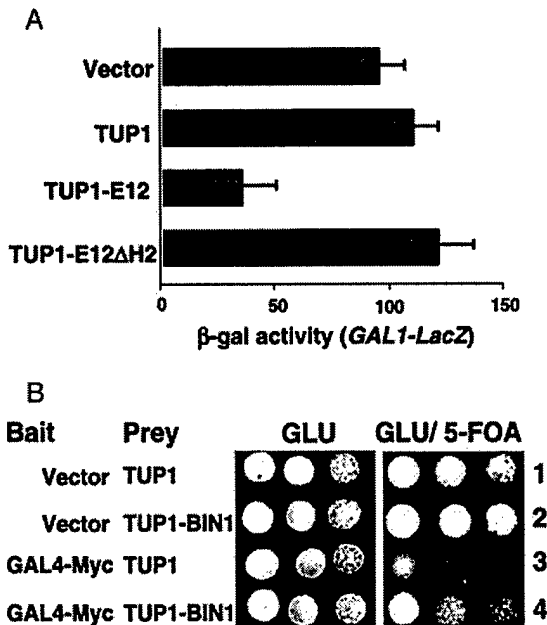
Fig. 5. RTA detects interactions with mammalian transactivators. (A) Yeast strain Y190 was cotransformed with pGAL4-MyoD and a vector control (pRS425), pRST425 expressing TUP1-RD, pRST425 expressing TUP1-E12, or pRST425ΔH2 expressing TUP1-E12 bearing a deletion of helix 2 (TUP1-E12ΔH2). Yeast was grown to mid-log arithmetic phase in selective medium containing glucose, and expression of the GAL1-lacZ reporter gene was assayed by measuring β-galactosidase activity. (B) Yeast strain MAV108 was transformed with the bait vector control plasmid (pG1), or pG-Myc(1-262) expressing GAL4-Myc, in combination with the prey vector control plasmid pBD1 (TUP1) or a pBD-BIN expressing TUP1-BIN1. Cells were spotted, in 10-fold serial dilutions (from left to right) on selective plates containing glucose without 5-FOA (GLU), or with 0.05% 5-FOA (GLU/5-FOA).
