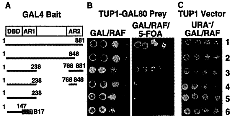
Fig. 4. Repression of GAL transcription by TUP1-GAL80 requires the GAL4 C-terminal 30 amino acids. (A) Fusion derivatives and deletions of GAL4. (B) Yeast strain yJM11 was cotransformed with pJM1107 expressing TUP1-GAL80 and plasmids expressing the GAL4 deletion/fusion derivatives indicated in A. Cells were spotted, in 10-fold serial dilutions (from left to right) on selective plates containing galactose and raffinose without 5-FOA (B, GAL/RAF), or with 0.1% 5-FOA (B, GAL/RAF/5-FOA). (C) Yeast cotransformed with GAL4 expression plasmids (indicated in A) and pJM1105 were spotted as above on minimal selective plates lacking uracil (URA - /GAL/RAF), to assay activation of the GAL1-URA3 reporter.
