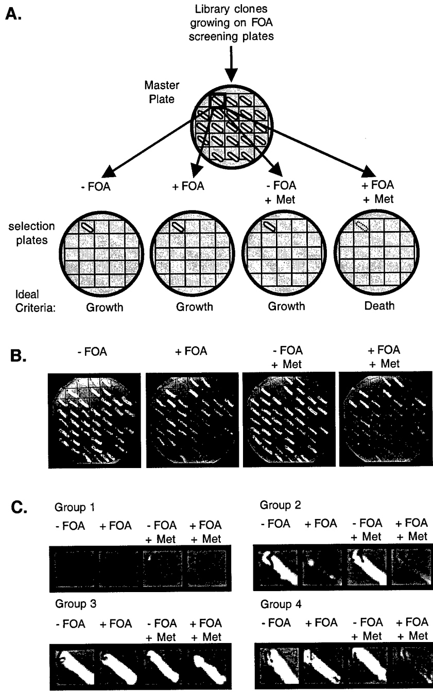
Figure 2 Identification of novel Myc NTD-interacting proteins by library screen using RTA (A) Schematic outline of library screen and selection criteria. FOA resistant colonies were collected and transferred from screening plates onto master plates. Library clones were then tested by directly transferring cells from master plates to a series of selective plates designed to test for specificity and recapitulation of growth phenotype on FOA. (B) A representative set of library selection plates. (C) Clones can be divided into 4 categories. Group 1 clones were viable when picked from original screening plates onto master plates, but were not viable when transferred from master plates to selection plates. Group 2 clones were viable on selection plates, but did not confer growth on FOA. Group 1 and 2 clones were not carried further. Group 3 clones were able to confer strong rescue on FOA, however, strong growth was also seen on +Met, suggesting that the growth on FOA could be non-specific. Group 4 clones exhibit the ideal selection criteria, rescue of growth on FOA and loss of this rescue when transferred to +Met indicating specificity of growth on FOA to the concurrent expression of the library TUP1-fusion.
