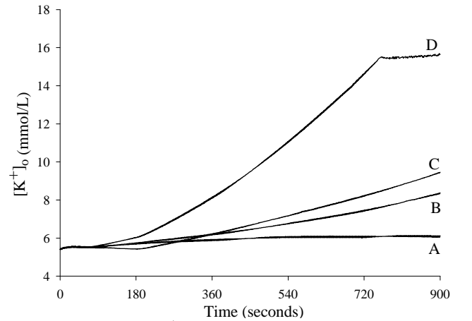
Fig. 2. Extracellular K^+ accumulation during simulated ischemia.
