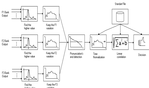
Fig. 2 – Block diagram of time normalization, mathematical and decision modules.
