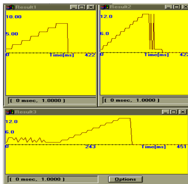
Fig. 4. – Formants extractor module's results to the test sweep, with duration of 300 ms. Each graphic represents a filter bank, and each axis represents the time and the number of the excited filter.
