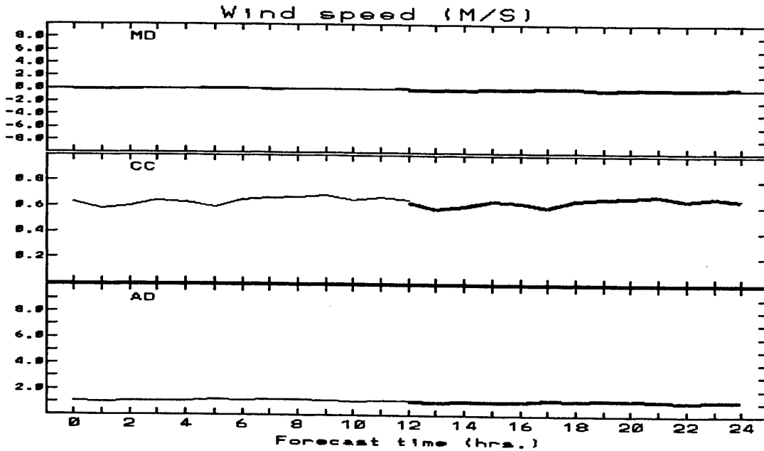
Figure 12(A). Time series of statistical parameters for wind speed between the nowcasted data and the observed data from both "S" and "*" sites.
