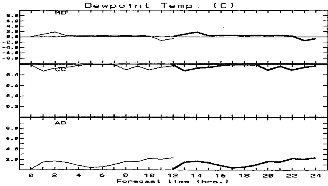
Figure 11(A). Time series of statistical parameters for dew point temperature between the nowcasted data and the observed data from both "S" and "*" sites.
