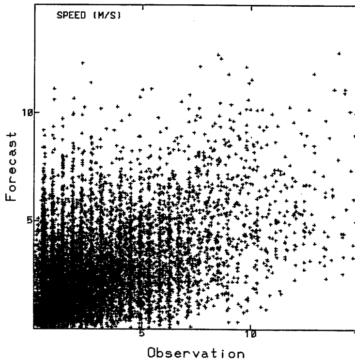
Figure 9. Wind speed comparison between the nowcasted data and the observed data.
