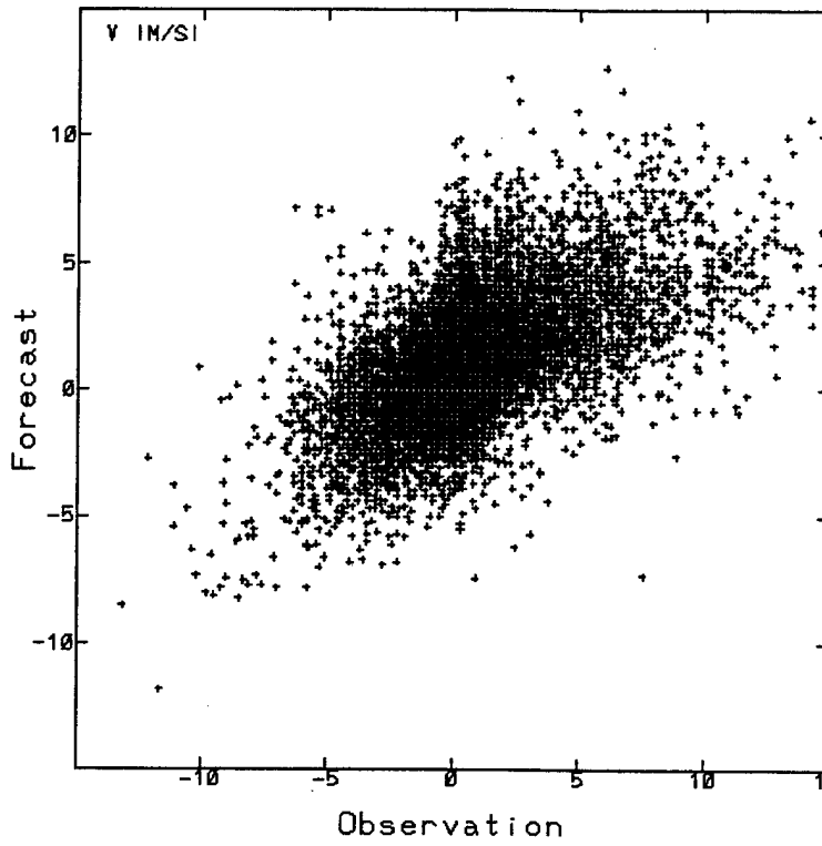
Figure 8. Wind vector-y component v comparison between the nowcasted data and the observed data.
