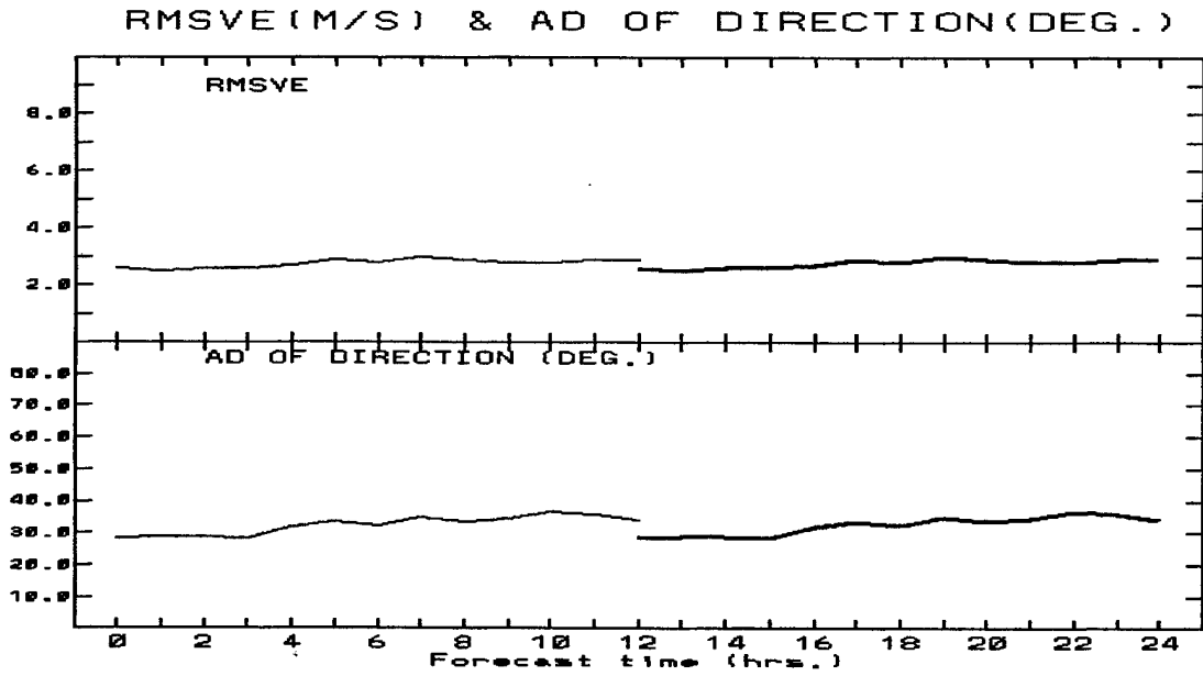
Figure 13(A). Time series of RMSVE and MWDDF between the nowcasted data and the observed data from both "S" and "*" sites.
