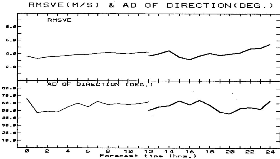
Figure 13(B). Time series of RMSVE and MWDDF between the forecast data by BFM and the observed data from both "S" and "*" sites.
