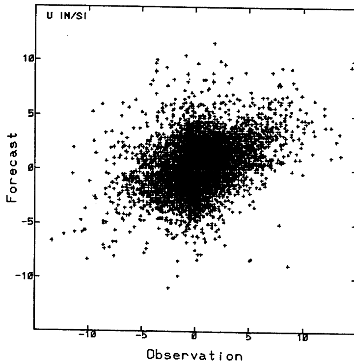
Figure 7. Wind vector-x component u comparison between the nowcasted data and the observed data.
