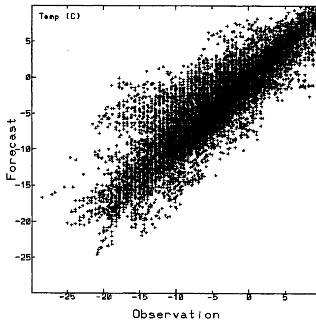
Figure 5. Temperature comparison between the nowcasted data and the observed data.
