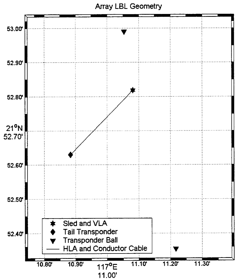
Figure 3-1: Location of the LBL system components. The tail transponder transmitted an 11.5 kHz interrogation signal. After the transponder balls received the interrogation, the north ball replied at 12.0 kHz and the south ball replied at 11.0 kHz. The time difference between the interrogation transmission and the reception of the three frequencies by the four LBL channels on the VLA and three LBL channels on the HLA was recorded to obtain positions.
