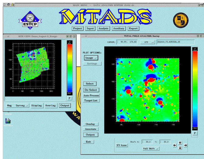
Fig. 6 – A working screen of the MTADS DAS showing the project view on the left and an expanded analysis window on the right
