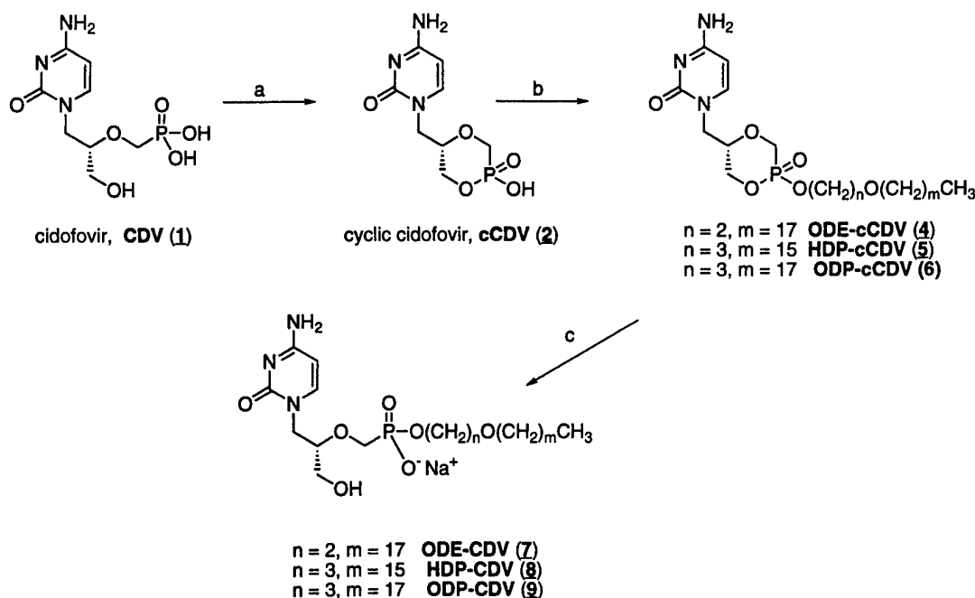
FIG. 1. Synthesis of alkoxyalkyl analogs of CDV and cCDV. Reagents: a, N,N -dicyclohexyl-morpholinocarboxamidine, 1,3-dicyclohexylcarbo-diimide, pyridine, 100°C; b, ODE-Br, ODP-Br, or HDP-Br, N,N -dimethylformamide, 80°C; c, 0.5 M NaOH. The underscored numbers in parentheses correspond to the compound numbers used throughout the report.
