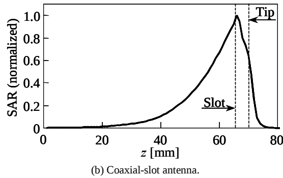
Fig. 7. SAR distributions.
