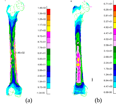
Fig. 2. Von Mises stress distribution in the intact femur at toe-off in (a) walking, and (b) in jogging
