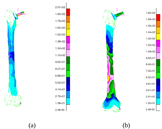
Fig. 3. Von Mises stress distribution in the nailed femur at toe-off in (a) walking, and (b) in jogging
