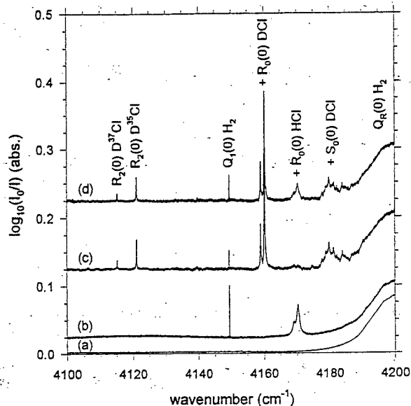
FIG. 7. Survey of HCl- and DCl-induced IR activity in solid p\text{H}_2 . Trace (a) is the spectrum ( 0.1 \text{ cm}^{-1} resolution) of a 3.1-mm-thick as-deposited 120 ppm o\text{H}_2/p\text{H}_2 solid at T = 2.4 \text{ K} . The very weak feature near 4153 \text{ cm}^{-1} is the Q_1(0) \text{ H}_2 absorption induced by residual o\text{H}_2 molecules; the broad feature at the right side of the spectrum is the rising edge of the Q_R(0) \text{ H}_2 phonon sideband. Trace (b) is for the as-deposited 88 ppm HCl/ p\text{H}_2 sample depicted in the upper panel of Fig. 2. Trace (c) is for the as-deposited 102 ppm DCl/ p\text{H}_2 sample depicted in the lower panel of Fig. 2. Trace (d) is for an as-deposited 2.9-mm-thick p\text{H}_2 sample doped with 50 ppm HCl and 100 ppm DCl at T = 2.5 \text{ K} ; 0.01 \text{ cm}^{-1} resolution. The sharp features in traces (b) through (d) near 4149.4 \text{ cm}^{-1} are the Q_1(0) \text{ H}_2 absorption transitions induced by the presence of HCl and DCl dopant molecules. The labels “+ R_0(0) \text{ DCl} ,” “+ R_0(0) \text{ HCl} ” # and “+ S_0(0) \text{ DCl} ” are shorthand for the Q_1(0) \text{ H}_2 + R_0(0) \text{ DCl} , Q_1(0) \text{ H}_2 + R_0(0) \text{ HCl} , and Q_1(0) \text{ H}_2 + S_0(0) \text{ DCl} cooperative absorptions in which the dopant molecules undergo a pure rotational transition. Traces (c) and (d) also show the R_2(0) \text{ DCl} vibrational overtone transition.
