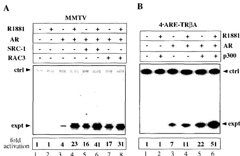
Fig. 7. Coactivators Such as SRC-1, RAC3, and p300 Stimulate Both Ligand-Dependent and -Independent Activation by AR
