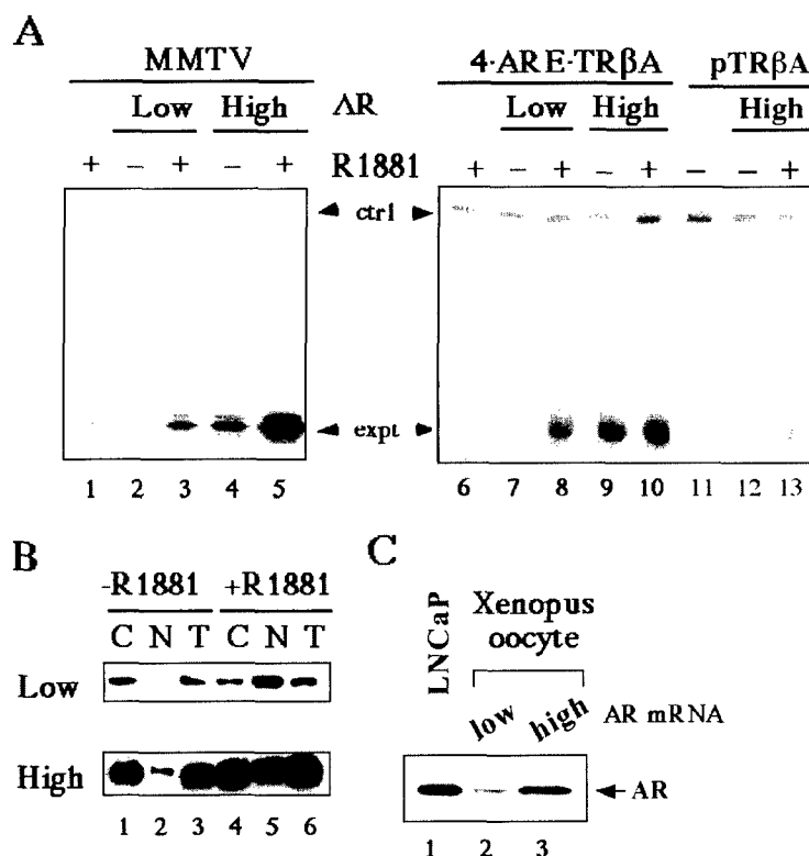
Fig. 3. AR Exhibits Both R1881-Dependent and -Independent Activation
