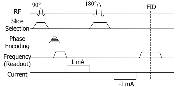
Fig. 2. Pulse sequence used in MRCDI
