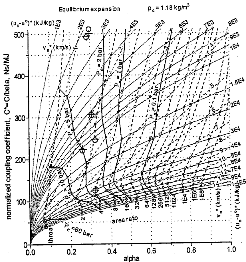
Figure 5. Isentropic expansions of laser heated STP air ( 1.18 \text{ kg/m}^3 ) from initial states of specific internal energy ranging from 1 to 110 MJ/kg. The circles and nearby crosses represent the blowdown quantities obtained from initial [u_c - u^0]^* states of 2E3, and 1E4 J/kg for the frozen expansion and 2E3, 6E3, 1E4, and 4E4 kJ/kg for the equilibrium expansion.
