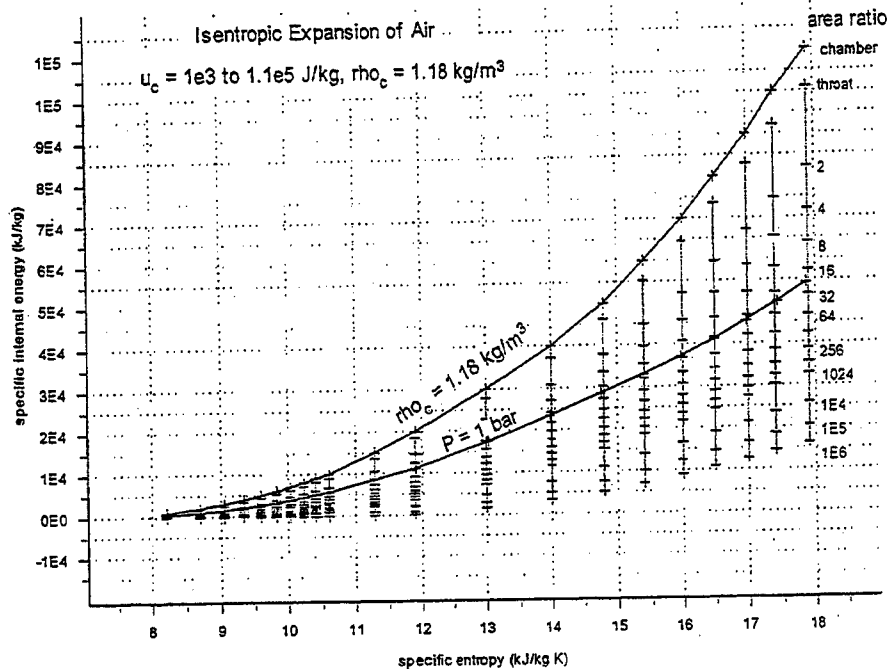
Figure 4. Isentropes for equilibrium expansions originating from the constant density line at 1.18 \text{ kg/m}^3 and terminating on the constant pressure line at 1 bar. Lines of constant area ratio are nearly coincident with lines of constant density.
