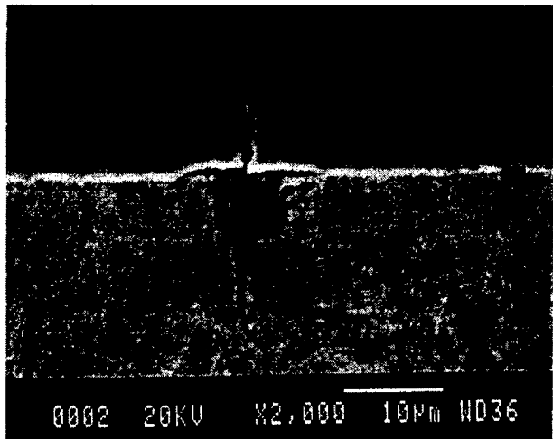
Figure 7. M829E3 enabling erosion example.
