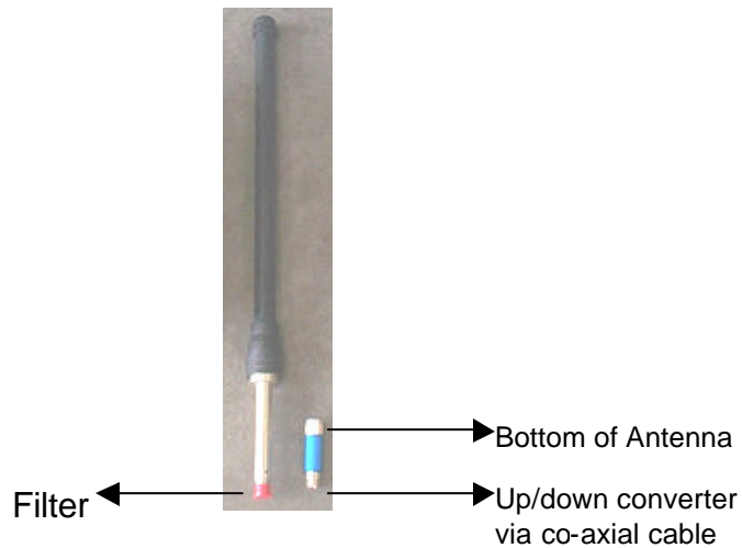
Figure 5: Connections – RF Relay Antenna & Filter
