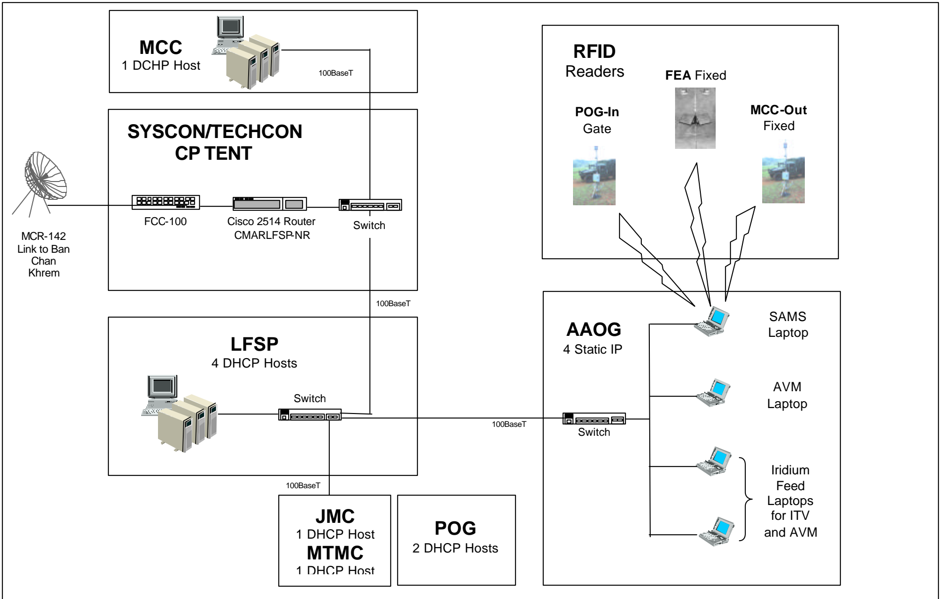
Figure 5: POG/MCC Network Architecture
