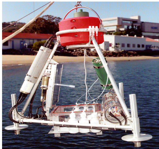
Figure 3. Benthic flux sampling device.
