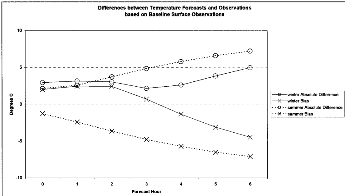
Figure 4. Baseline temperature forecast accuracy by forecast hour.
