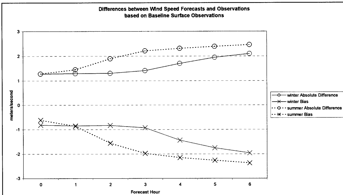
Figure 6. Baseline wind speed forecast accuracy by forecast hour. Note: Negative bias when forecast is too low.
