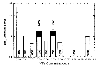
Figure 2. Grain Size vs YTa content, y . Numbers denote sinter temperature, T_s(^{\circ}\text{C}) .
