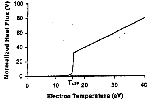
Fig. 2. Normalized heat flux to the wall versus electron temperature for xenon on boron nitride.
