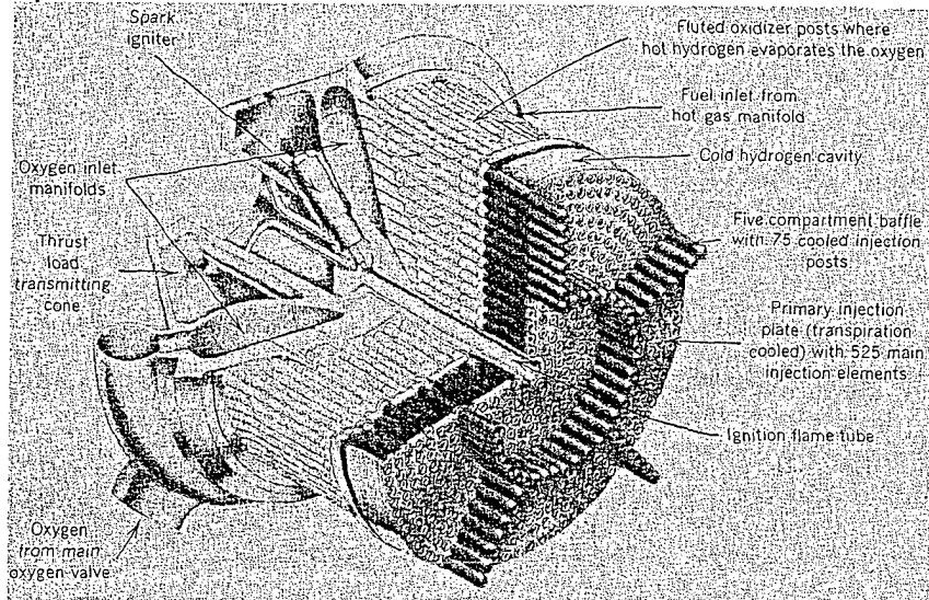
From Sutton, "Rocket Propulsion Elements," 6th ed., pg 277, Wylie 1992
