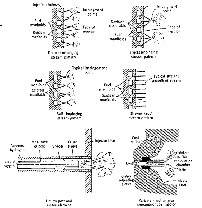
From Sutton, "Rocket Propulsion Elements," 6th ed., pg 299, Wylie 1992
