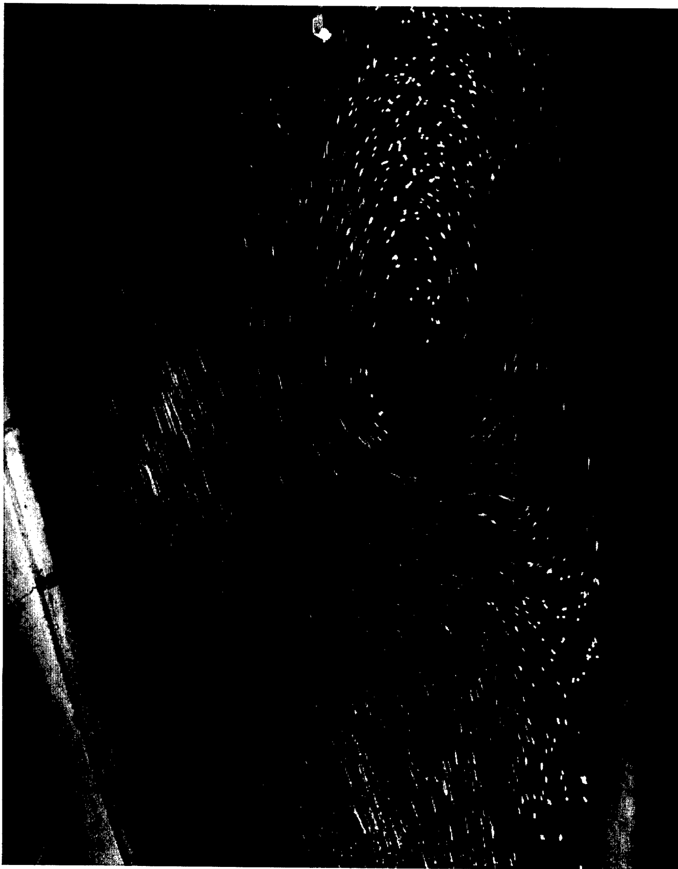
Photo 10. Confetti pattern, Plan A condition, 150,000 cfs
