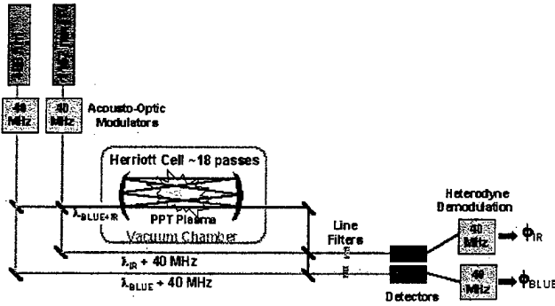
Figure 3: Interferometer Layout
