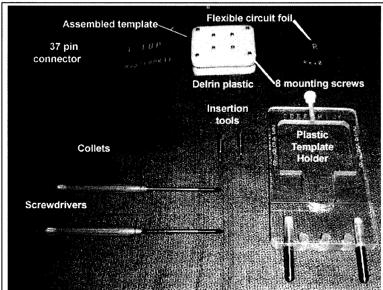
Figure 3: Assembled template and accessories. An assembled template is shown at the top of this figure, which is comprised of two connectors and the flexible circuit foil for attachment to the computer system for power control input and the two plastic components. The holes for the brachytherapy/hyperthermia needles are unique in that these needles cannot be inserted inadvertently into a thermometry hole. After the implantation of all brachytherapy/hyperthermia needles (usually 12-25) unused holes can be used for thermometry catheters in addition to the dedicated thermometry holes. The use of Delrin for the plastic template components represents a second-generation template. The original design used Lucite, which tended to crack after extended use probably as a result of cleaning fluids, gas sterilization and slightly non-uniform tightening of the template screws. During the implant procedure the template itself is mounted into the plastic template holder which in turn is mounted onto the real time ultrasound unit providing a fixed reference while inserting needles and thermometry catheters. Brachytherapy/hyperthermia needles (Figure 4) are assembled during the implant procedure with a custom insulator placed on the needle to protect tissues intervening between the surface of the template and the proximal aspect of the tumor. The template is designed such that when the eight clamping/tightening screws in the template are loose the needle with insulator installed can pass through but cannot come back out. Prior experience with LDR templates demonstrated that the insulators are an essential feature to protect the tissues of the perineum, decrease pain and improve patient tolerance. The actual thermometry devices (usually consisting of 5 discrete points at 1 cm. separation) are inserted later in the patient's room at the beginning of the first hyperthermia session. The number of thermometry catheters placed is expected to vary from 4 to 8 depending on the implant, and up to 32 sensors can be implanted in these catheters. All components shown here, and in Figure 4 below, are gas sterilized prior to an implant procedure
