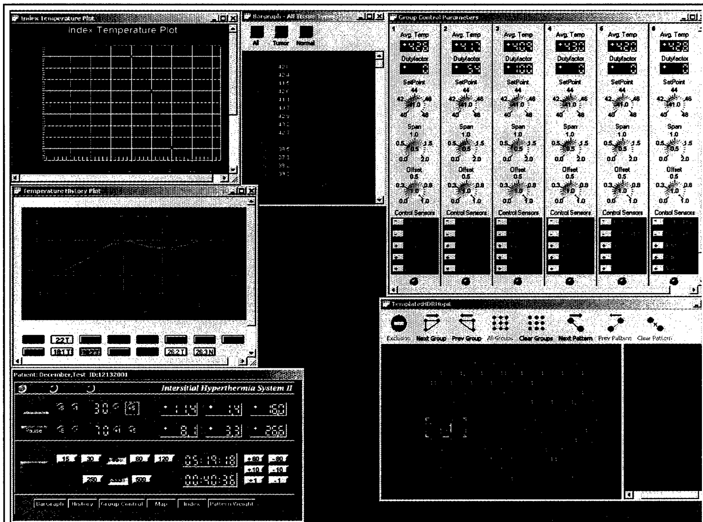
Figure 7: Screen capture of an alternate display arrangement to that shown in Figure 6 taken on the same phantom at a different time. At the upper right the complete group control panel (GCP) is shown. This control pane permits alteration of the power control algorithm parameters for each group of needles. In this particular case there are six groupings of needles. Individual needles may be members of any number of groups and groups can consist of as few as two needles. This grouping and control arrangement is essential to controlling power adequately to the essentially random spacing and patterns used in typical HDR implants. The implant pattern is determined by optimizing the brachytherapy dose distribution. No alteration of the pattern is done to accommodate hyperthermia administration although we anticipate that it may be necessary to add one to three needles to some implants to optimize hyperthermia as well.
