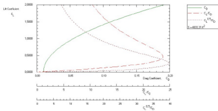
Figure 2.3 The drag polar for the clean airplane of 'alternative 1'
