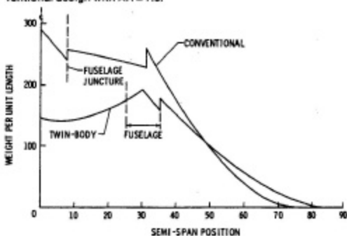
Figure 4 Wing load-carrying weight (ref. [1])
