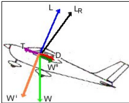
Figure IV.1 The forces acting on a plane in climb
