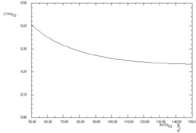
Figure 1.11 The results for the manoeuvring sizing
