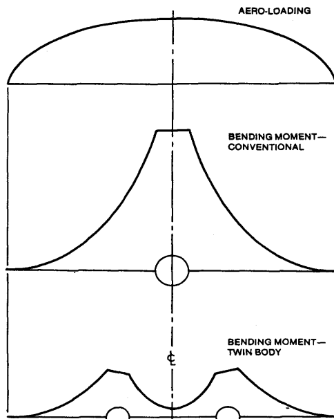
Figure 2 Twin fuselages reduce the peak bending moment (ref. [1])
