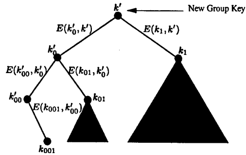
Fig. 2. Key revocation in the basic scheme.
