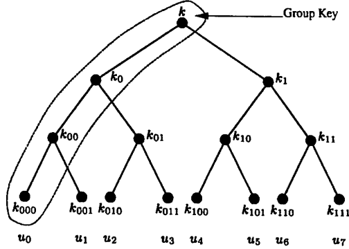
Fig. 1. The tree key data structure (the keys of u_0 are encircled).
