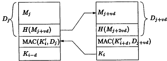
Figure 2: Immediate authentication packet example. D_j = H(M_{j+vd}) \parallel M_j and D_{j+vd} = H(M_{j+2vd}) \parallel M_{j+vd} .
