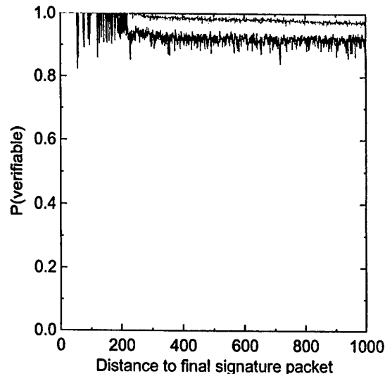
Figure 10. The verification probability for the basic vs. the extended scheme. Top line is the extended scheme. Bottom line is the basic scheme.
