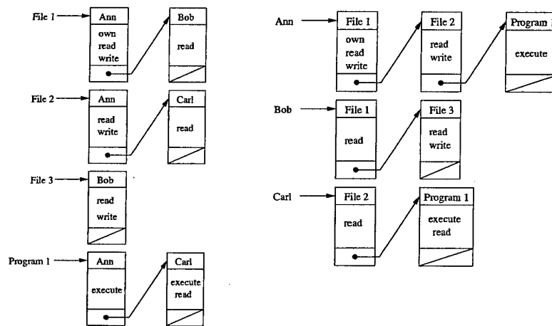
Fig. 3. Authorization table, ACLs, and capabilities for the matrix in Figure 1
