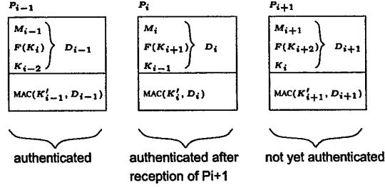
Figure 1. Basic stream authentication scheme. M_i stands for message i , P_i is packet i , K_i denotes the secret key i , F, F' are pseudo-random functions, and \text{MAC}(K'_i, D_i) computes the MAC of packet i using the secret key K'_i = F'(K_i) .
