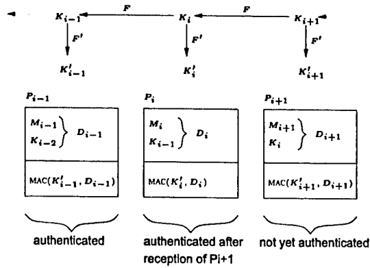
Figure 2. Scheme II. The packet format is the same as in scheme I, except that the commitment F(K_{i-1}) is omitted and the keys form a one-way key chain.
