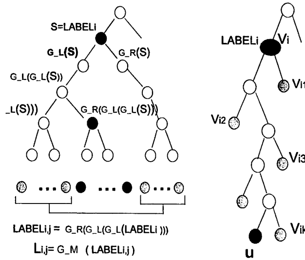
Figure 3: Key Assignment in the Subset Difference Method. Left: generation of \text{LABEL}_{i,j} and the key L_{i,j} . Right: leaf u receives the labels of v_{i_1}, \dots, v_{i_k} that are induced by the label \text{LABEL}_i of v_i .
