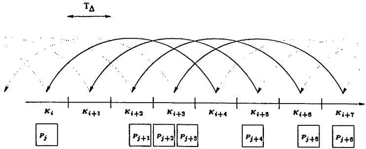
Figure 3. Scheme IV. The MAC key and disclosed key are only dependent on the time interval. The authentication key of P_j is K_i which is disclosed by packets sent during interval i + 4 . In this case, packet P_{j+4} discloses key K_{i+1} which allows the receiver to compute K_i and to authenticate packet P_j . We would like to point out that packets P_{j+2} and P_{j+3} are both authenticated with the same MAC key K'_{i+3} , because they were sent in the same time interval.
