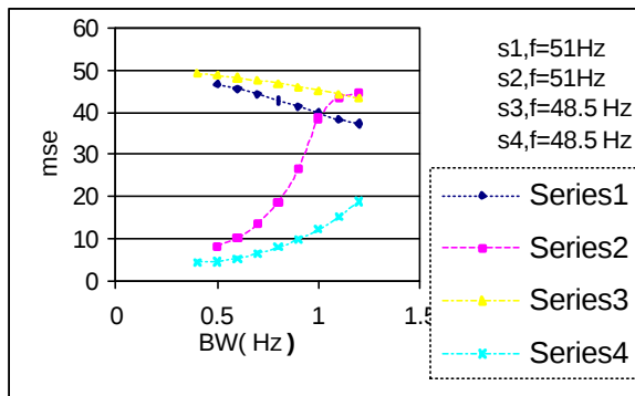
Fig. (10) Comparison of adaptive and non-adaptive IIR notch filters at frequencies of 48.5 Hz and 51 Hz.
