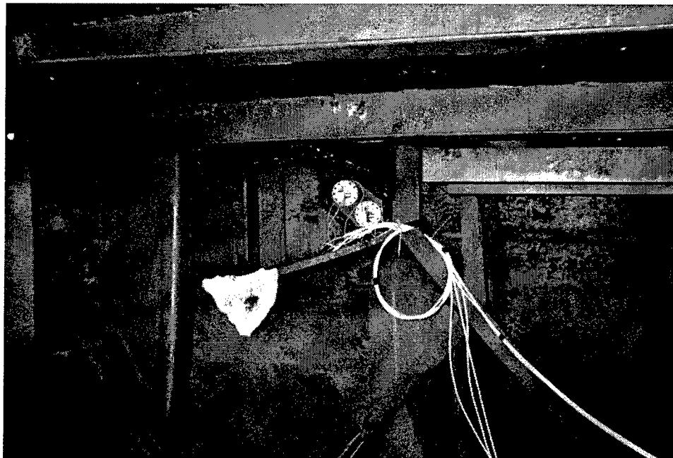
Figure 11. Accelerometers installed under deck
