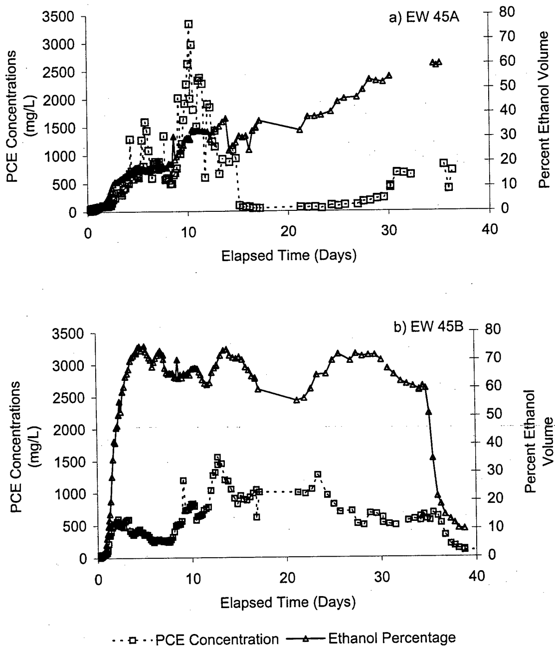
Figure 2 PCE concentrations and ethanol percentages from a) upper zone extraction well EW 45A, and b) lower zone extraction well EW 45B.
