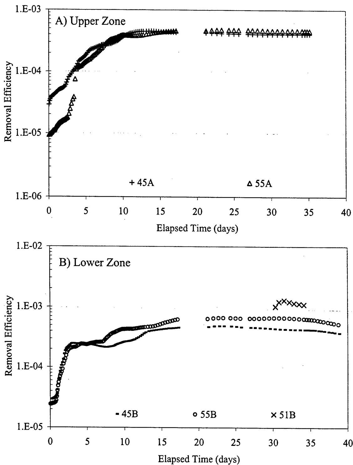
Figure 4 Removal efficiency as a function of elapsed time. Removal efficiencies are calculated as the cumulative PCE volume removed per cumulative extracted volume.
