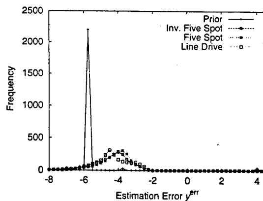
Figure 8. Estimation error Y^{err} of the NAPL block in the three pumping configurations.
