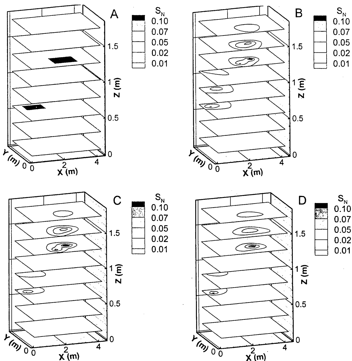
Figure 7. Estimates of NAPL block field. (a) True field. (b) Estimate produced in inverted double five-spot configuration. (c) Estimate produced in double five-spot configuration. (d) Estimate produced in line-drive configuration.
