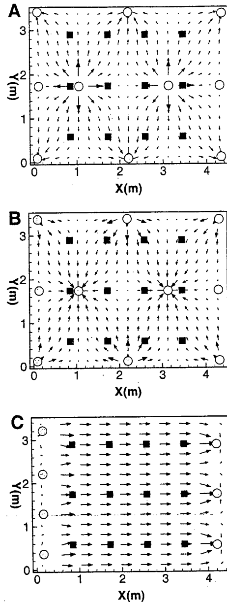
Figure 1. Plan views of the three pumping configurations tested. Squares represent locations of multilevel samplers (MLS), and circles represent locations of wells. Vertical spacing of the MLS locations are approximately 0.38 m. (a) Inverted double five-spot pattern. (b) Double five-spot pattern. (c) Line drive system.
