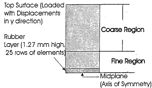
Figure 3: Explanation of Mesh and Boundary Conditions
