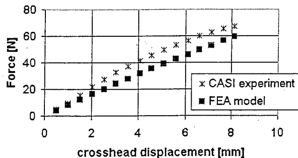
Figure 4: Load vs. Displacements in Experiment and FEA Model
