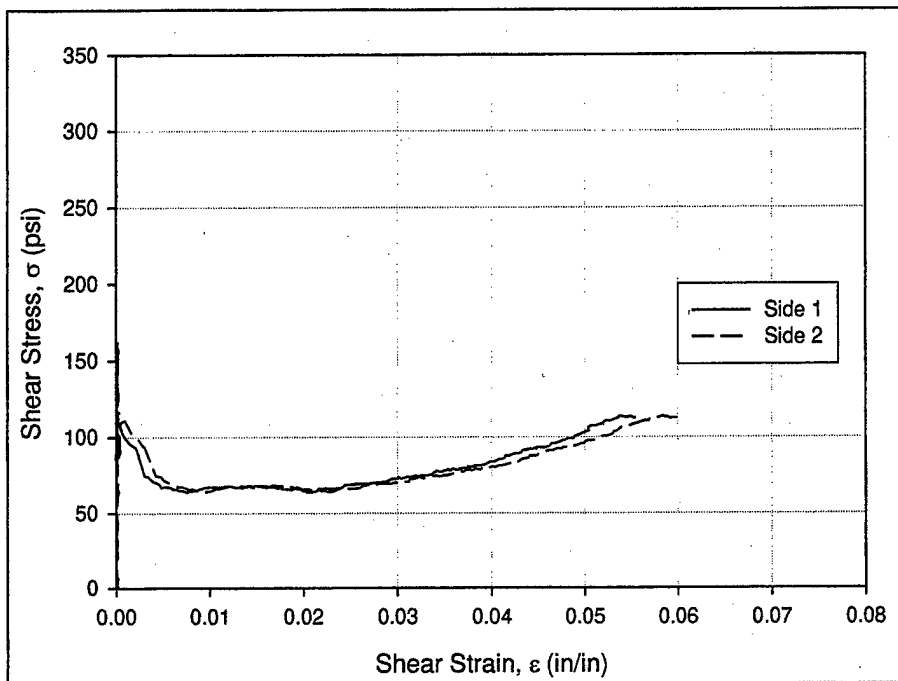
Figure 34. Stress-strain behavior of O-LVDT, Sample 2.
