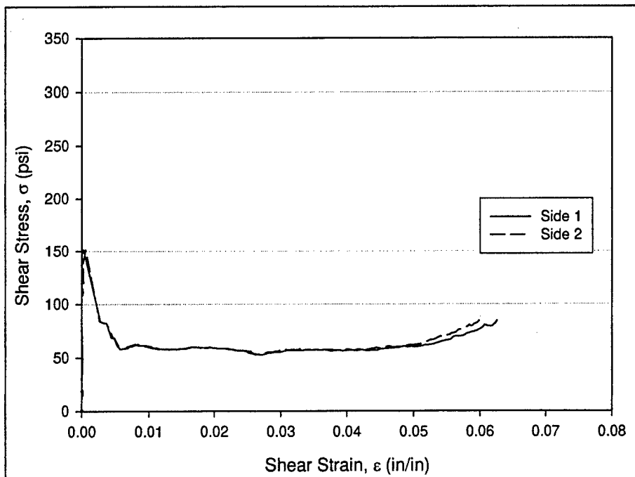
Figure 33. Stress-Strain Behavior of O-LVDT, Sample 1.
