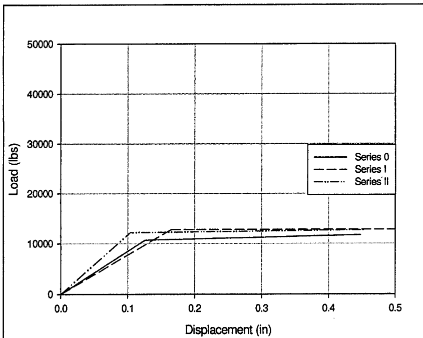
Figure 41. Idealized bilinear curve fit for Series 0, I, II at 12.5% normal load.
