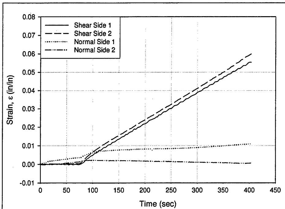
Figure 28. Normal and shear strain vs time of O-LVDT, Sample 2.
