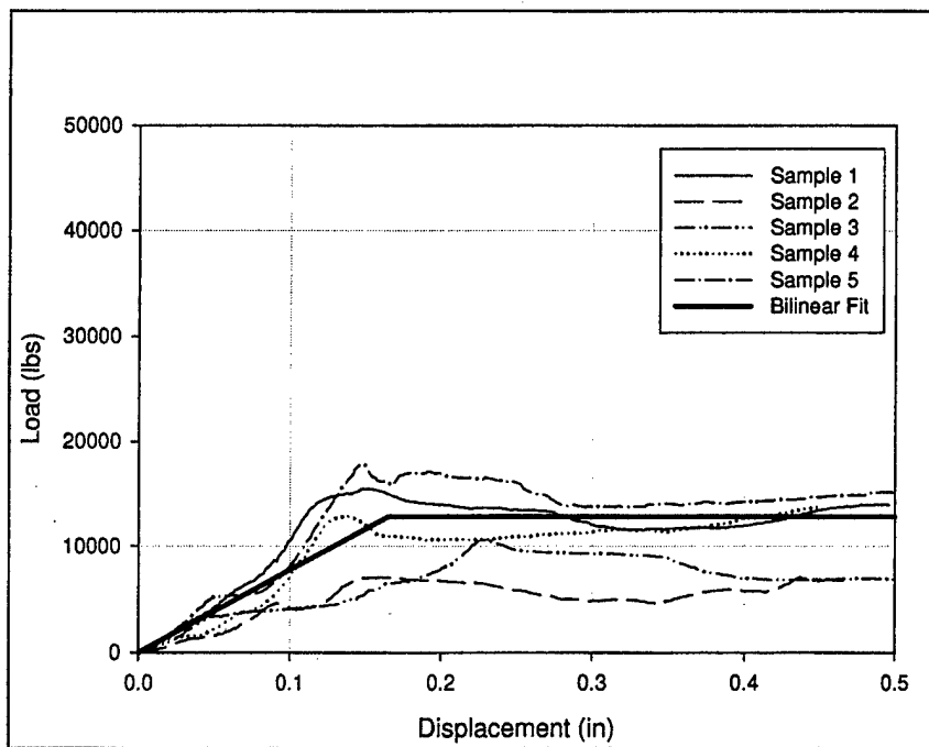
Figure 17. Load-displacement curves of I-12.5 group.
