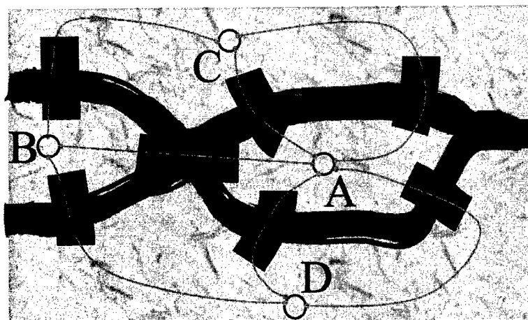
Figure 3.5: Königsberg Bridge Problem
