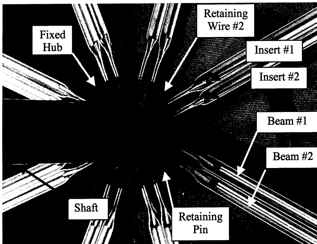
Figure 7.6: Umbrella Fixed Hub Structure
