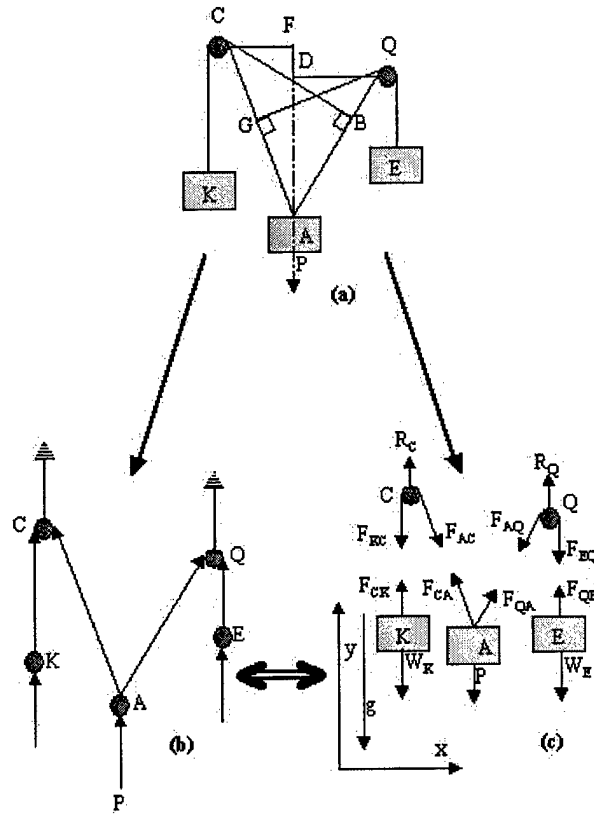
Figure 3.13: Equivalence of Free-Body Diagram (b) and Effort Flow Diagram (c) from Roberval's Apparatus (a)
