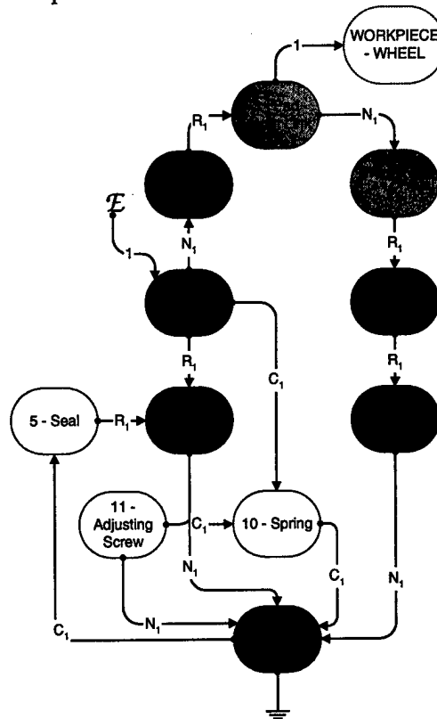
Figure B.3: 4-Bar Mechanism as Shown in Effort Flow Diagram
