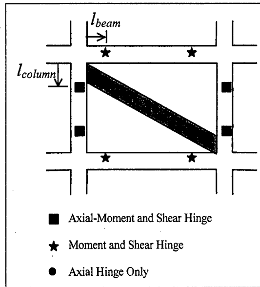
Figure A.6. Plastic hinge placement.
