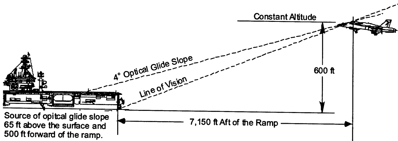
Figure 24: FOV Geometry
