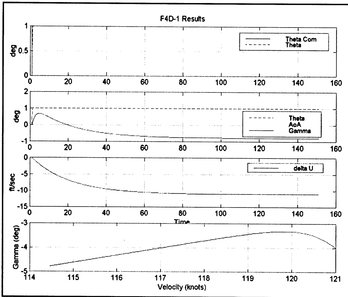
Figure 30: F4D-1 Flightpath Stability Analysis Results
