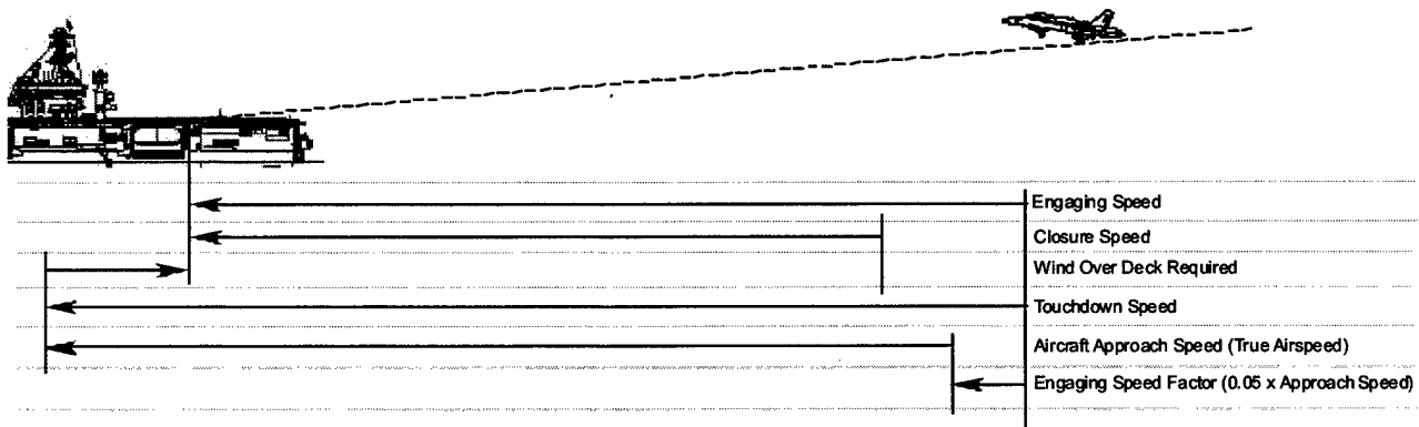
Figure 33: Speed Relationships
