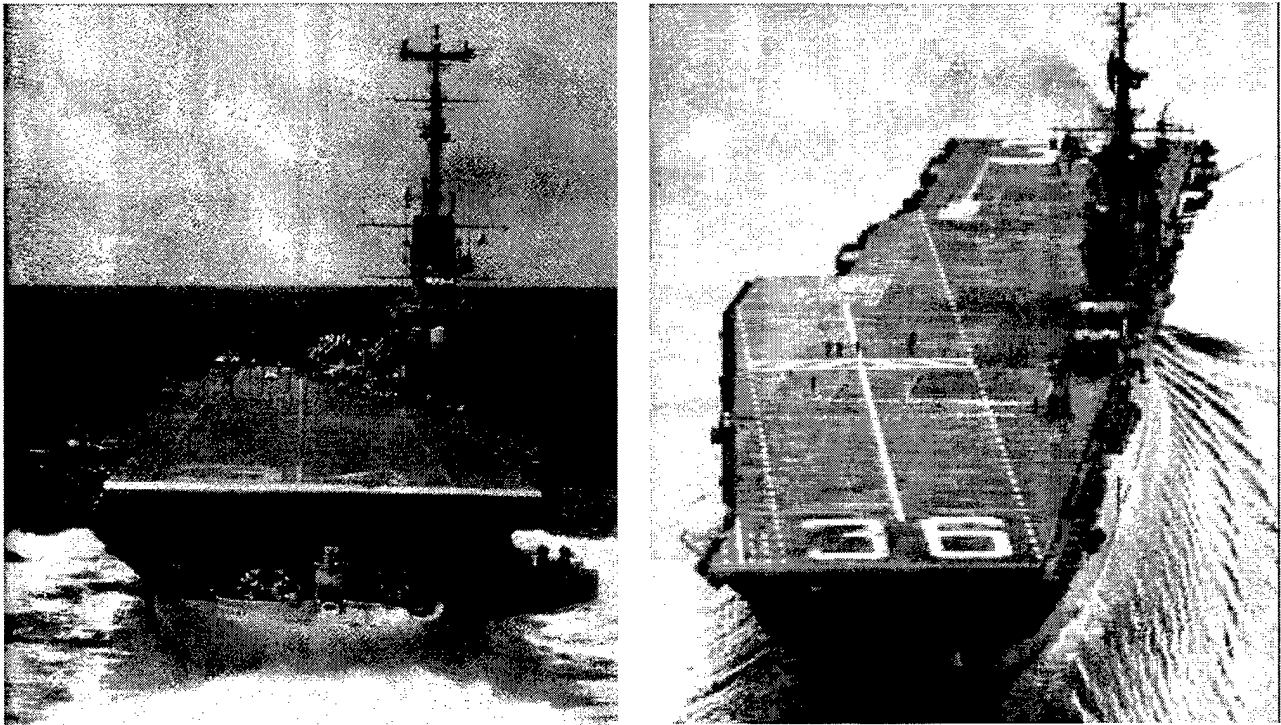
Figure 4: Straight Deck and Angled Deck Comparison View
