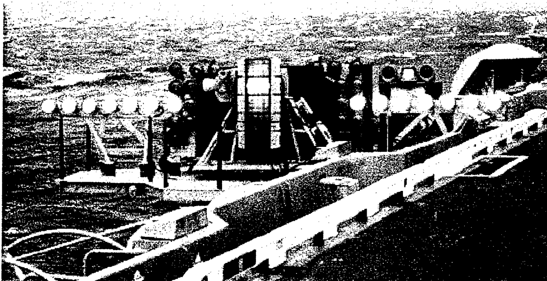
Figure 13: FLOLS
