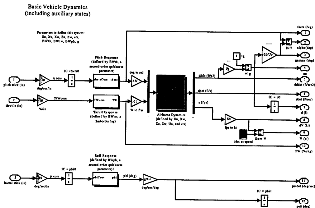
Figure C-4: Simulink Model of Aircraft Equations of Motion
