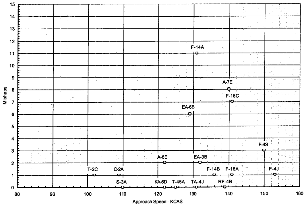
Figure 19: Mishaps versus Approach Speed (January 1980 - May 2001)
