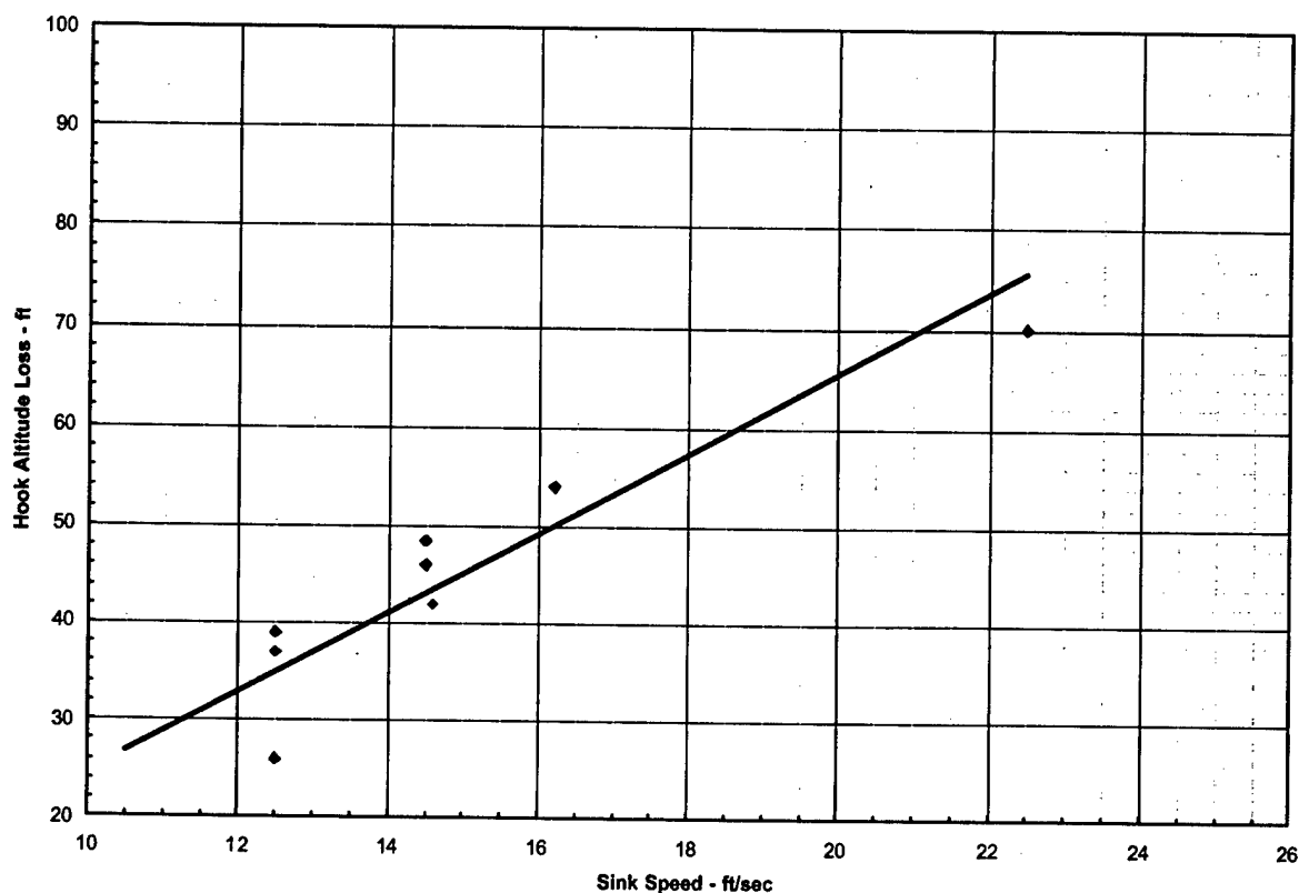
Figure 28: Hook Altitude Loss during Waveoff versus Sink Speed of Legacy Aircraft
