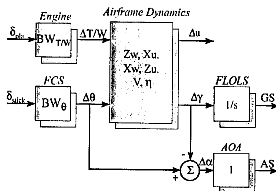
Figure C-2: Partitioned Model of Longitudinal Aircraft Dynamics.
