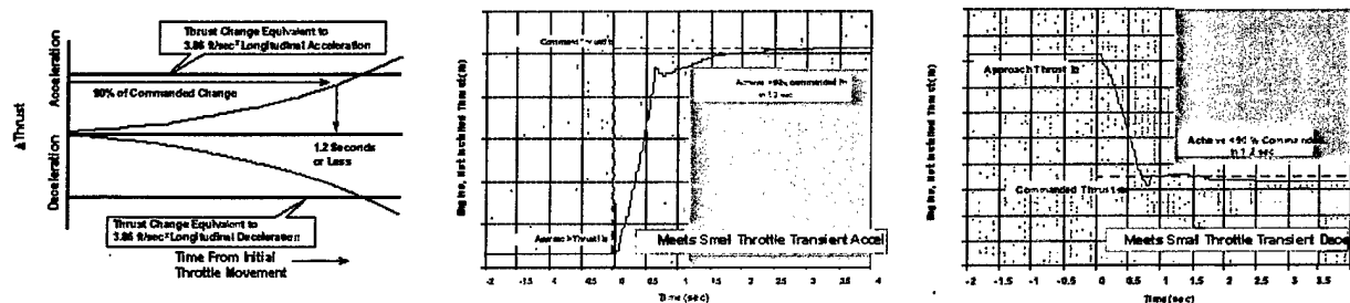
Figure 27: Small Throttle Transient Criterion
