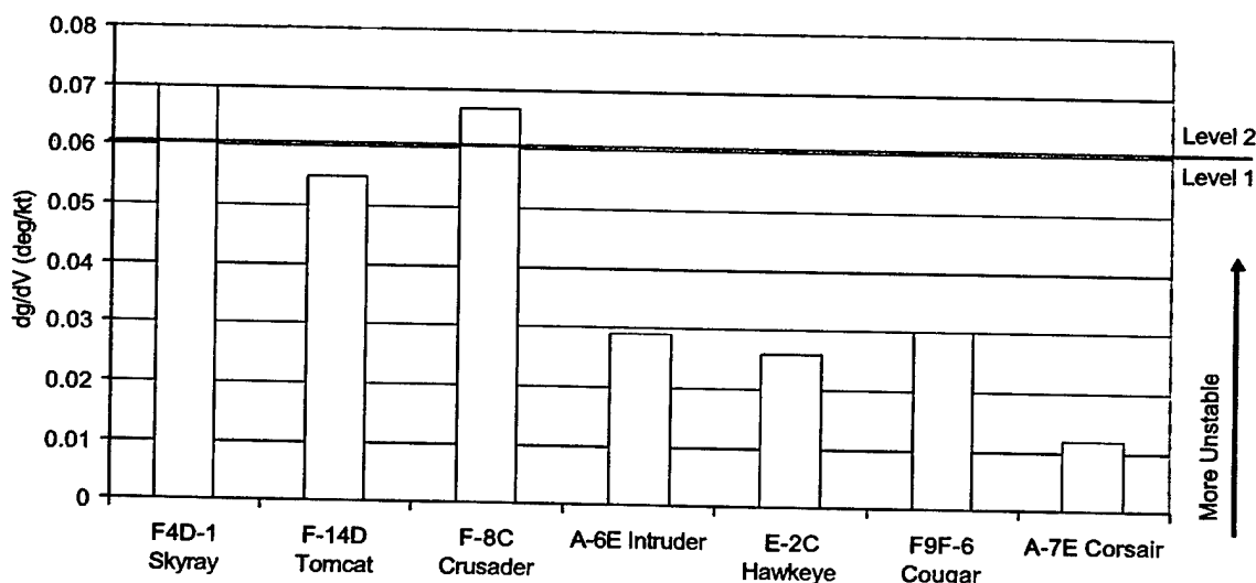
Figure 26: Flightpath Stability Characteristics of Selected Legacy Aircraft
