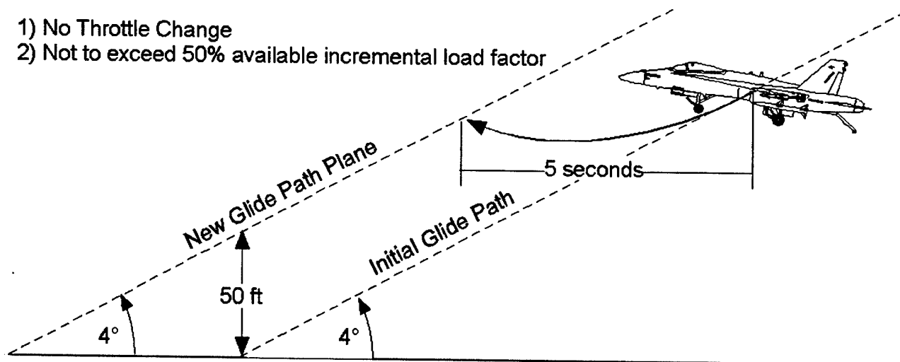
Figure 23: GS Transfer Maneuver
