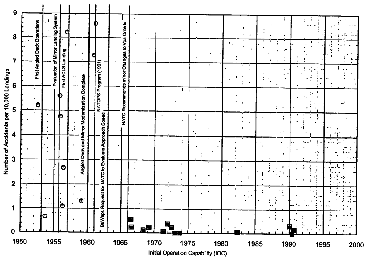
Figure 22: Historical Comparison of Mishap Rate and Key Milestones
