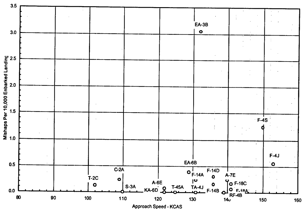
Figure 20: Mishaps per 10,000 CV Landings versus Approach Speed (January 1980 - May 2001)
