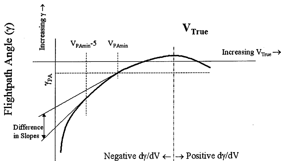
Figure 25: Flightpath Stability
