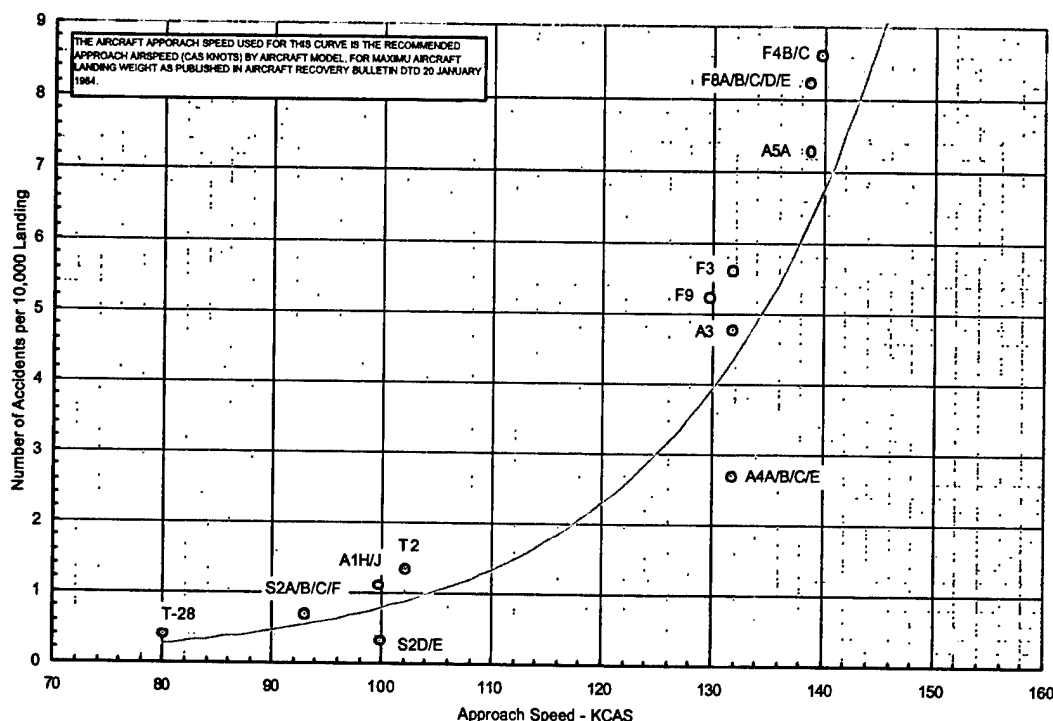
Figure 17: Vpa versus Aircraft Mishaps per 10,000 Landings (1964)
