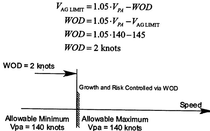
Figure 36: Controlling Risk and Growth through WOD Selection
