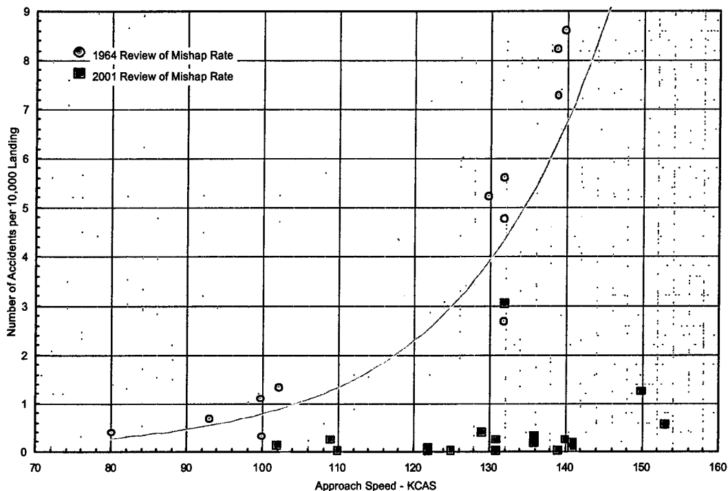
Figure 21: CV Approach Mishap Data Comparison (1964 versus 2001)
