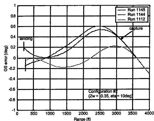
Figure C-8: GS Error Measured for Three Approaches
