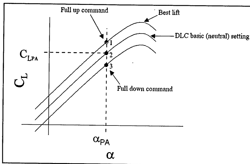
Figure 15: Direct Lift Control
