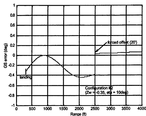
Figure C-9: GS Error following a Forced Offset
