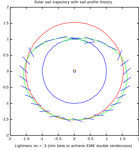
Figure 39 Trajectory for Minimum \beta EME Double Rendezvous
