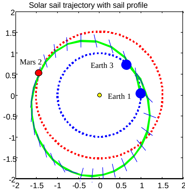
Figure 35 Single Cycle Path of Solar Sail Cyclor with Minimum V_{\infty}|_{\text{mars}}
