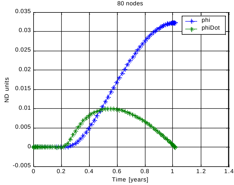
Figure 48 Optimal Profile for \mathbf{f} and \mathbf{w}_f States in the 3D Rendezvous Mission.
