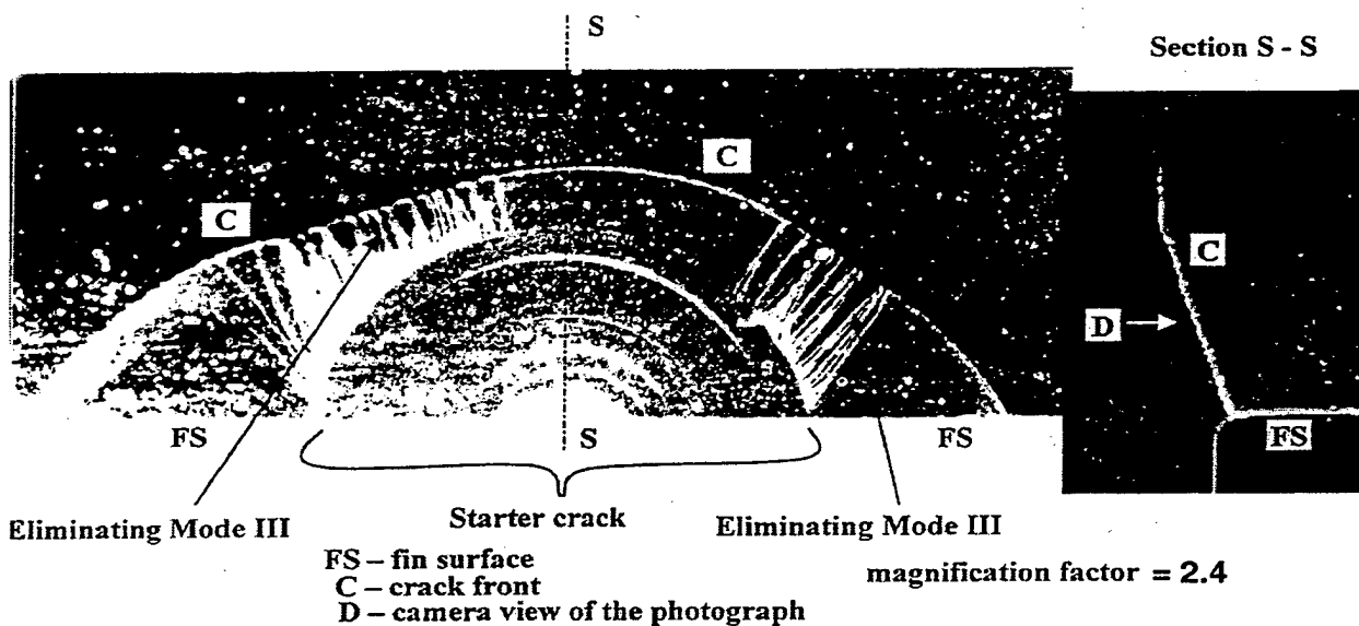
Model 8 Off-Axis Inclined Crack Showing Starter Crack and Final Mode I Crack Front
