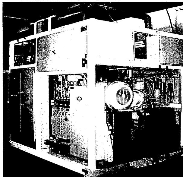
Compressor End
