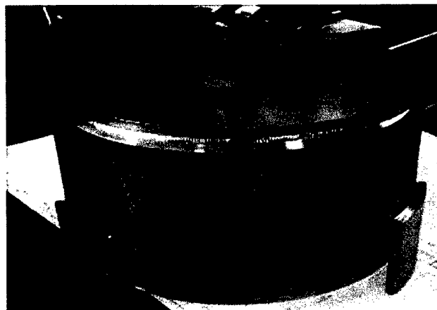
Fig. A-4 – Full-Scale Bonded Platinum Liner Test Article
