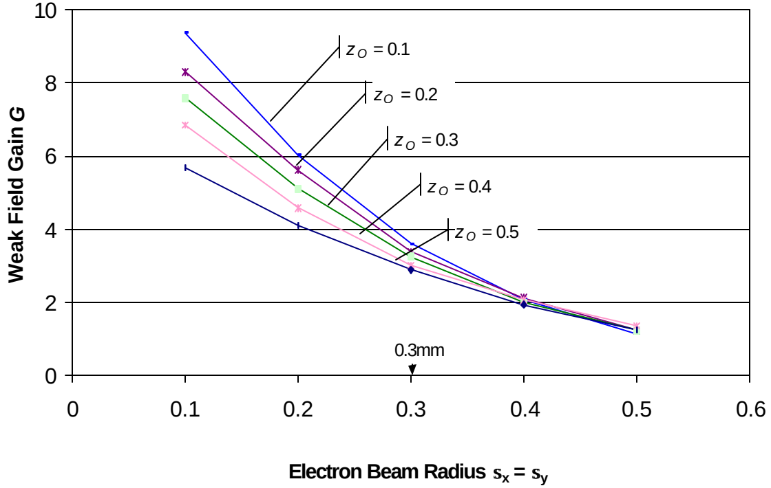
Figure 35. Weak Field Gain vs. Electron Beam Radius
