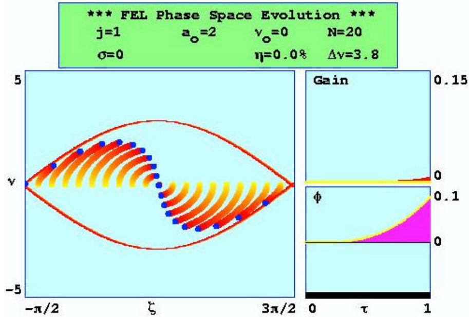
Figure 24. FEL phase space evolution at resonance
