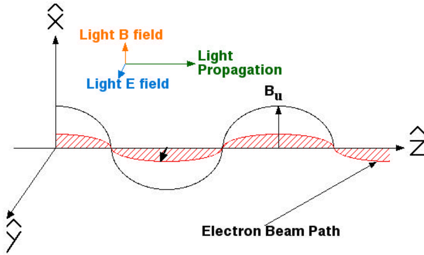
Figure 20. Electron Wiggle as a Result of the Undulator Field
