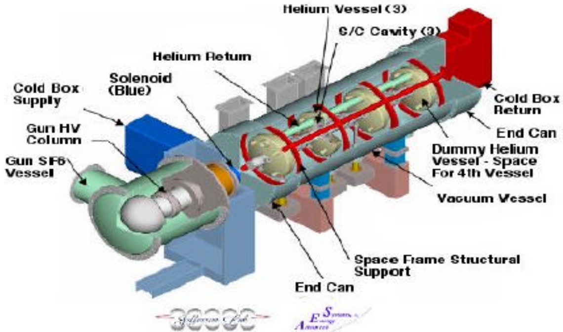
Figure 19. High average current photoinjector
