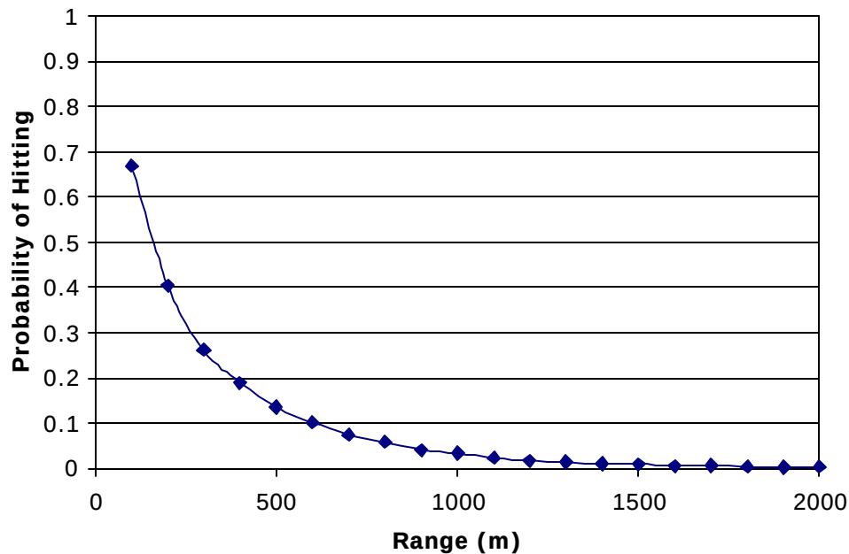
Figure 1. Probability of Missile Fragments Hitting the Ship
