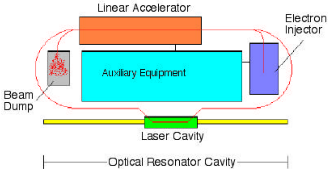
Figure 2. Oscillator Type Free Electron Laser with Energy Recovery in a Ring Configuration
