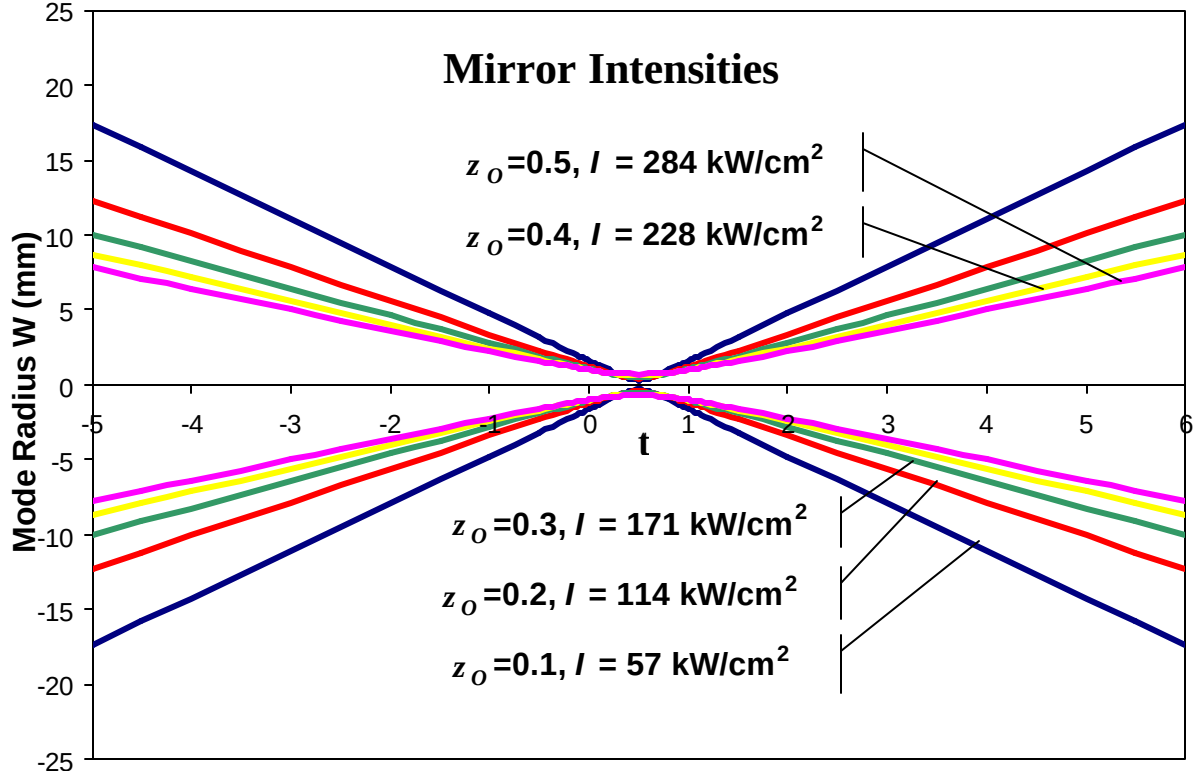
Figure 30. Spot Size Picture
