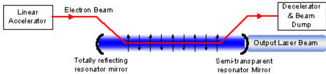
Figure 3. Oscillator Type Free Electron Laser Cavity
