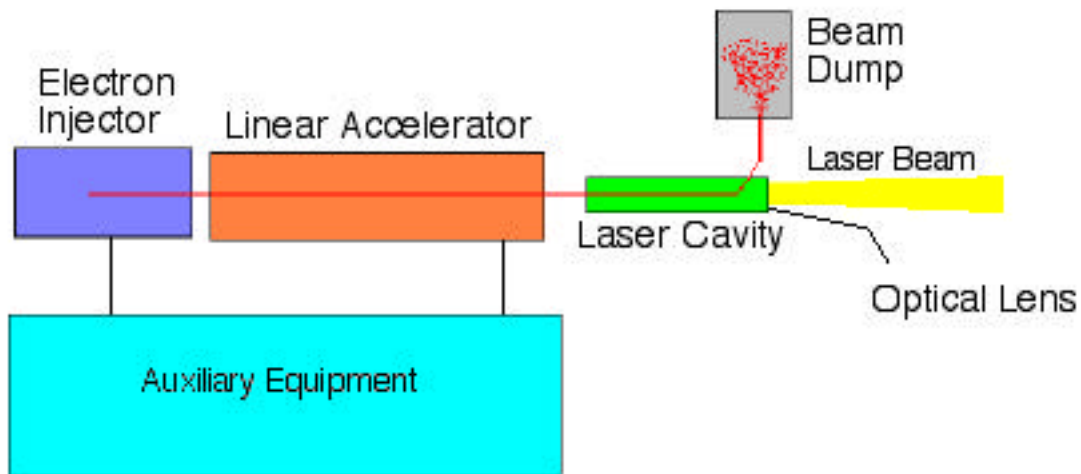
Figure 5. Amplifier Type FEL
