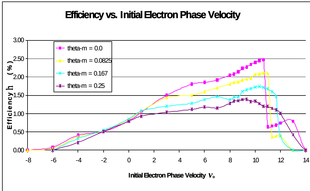
Figure 39. Efficiency vs. Initial Electron Phase Velocity as a Function of Mirror Tilt q_m
