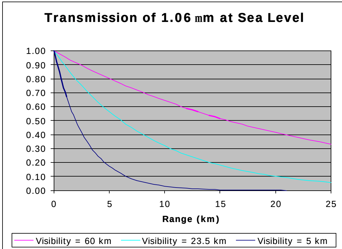
Figure 18. Transmission of 1.06 \mu\text{m} light at sea level for various atmospheric conditions
