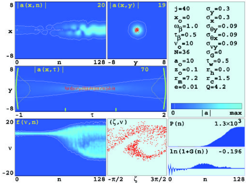
Figure 32. Extraction Efficiency Simulation
