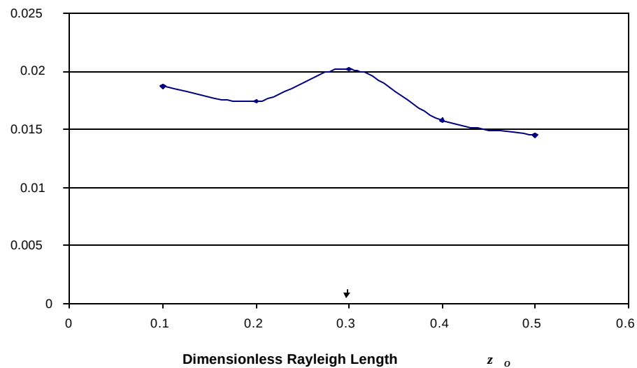
Figure 37. Peak FEL Efficiency vs. Rayleigh Length at Any Electron Beam Radius
