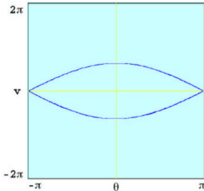
Figure 43. Pendulum separatrix
