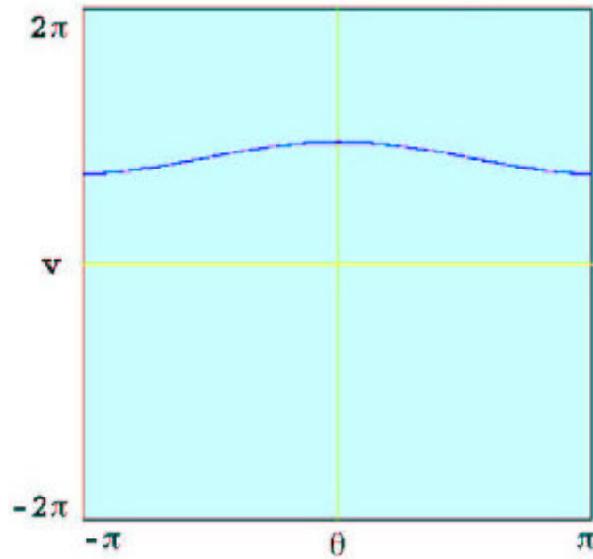
Figure 44. Simple pendulum open-orbit phase space plot
