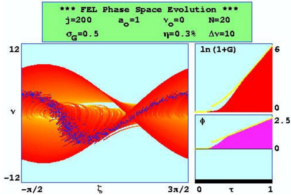
Figure 29. High current FEL phase space evolution
