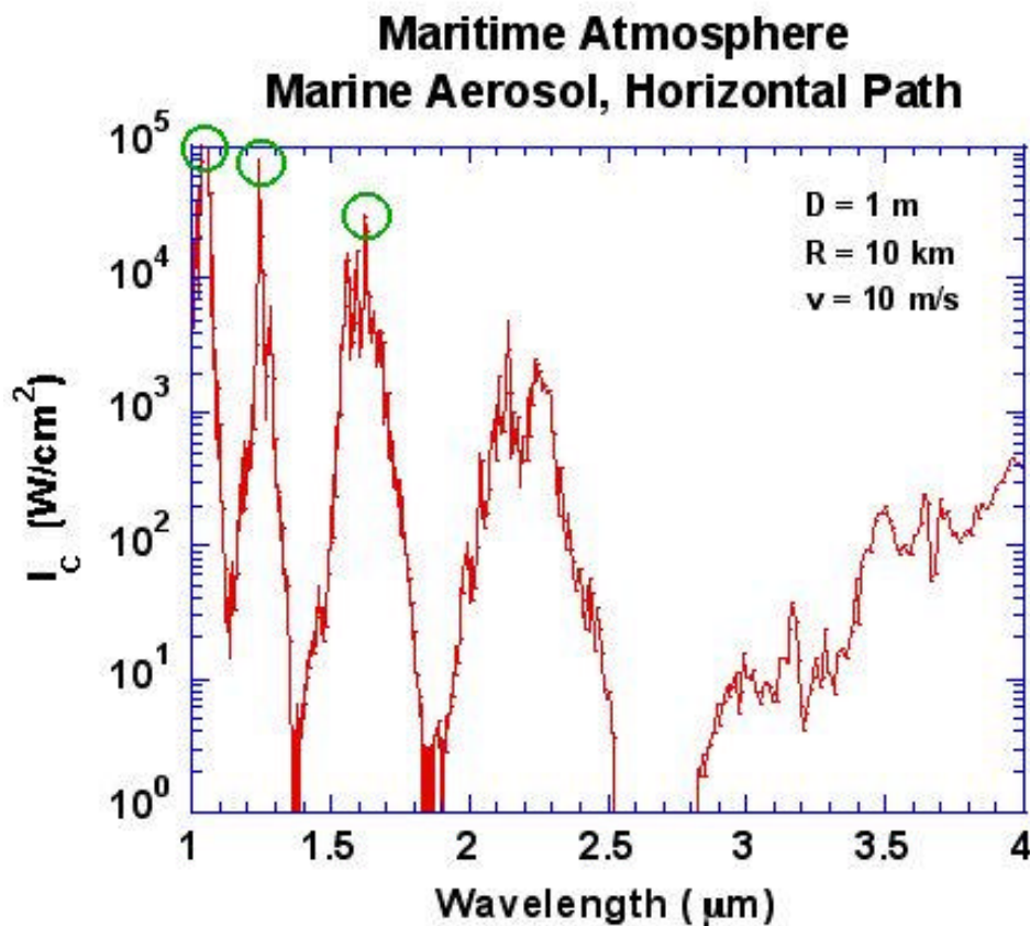
Figure 16. Transmittable intensity through a maritime atmosphere
