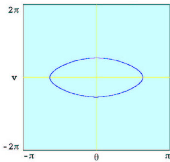
Figure 42. Simple pendulum closed-orbit phase space plot
