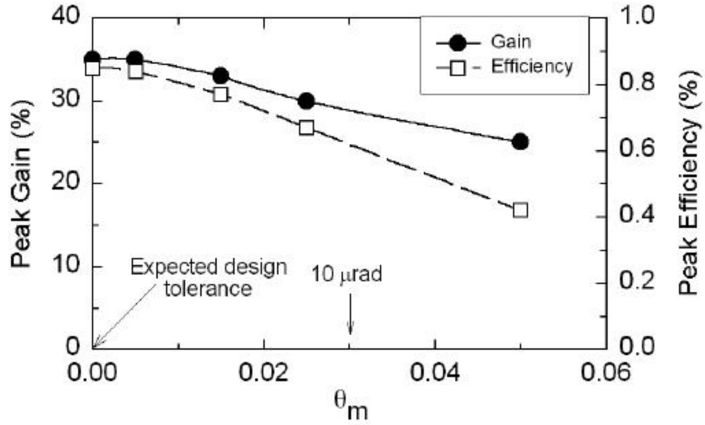
Figure 41. 100 kW Tilted Mirror Efficiency and Gain
