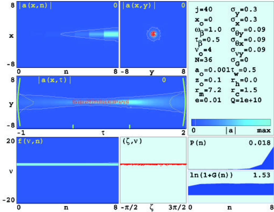
Figure 31. Weak Field Gain Simulation
