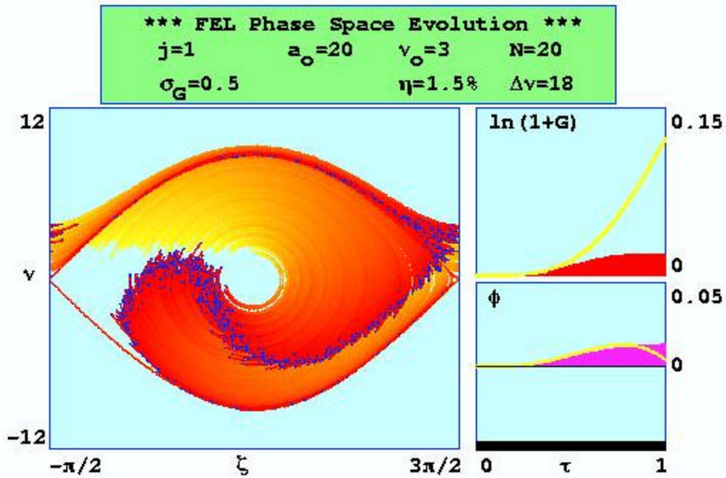
Figure 27. Strong field FEL phase space evolution
