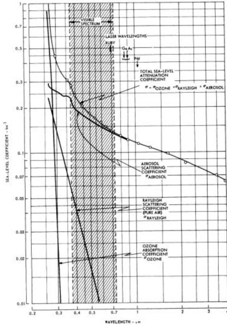
Figure 13. Atmospheric extinction coefficients for horizontal transmission at sea level with 23.5 km visibility. Absorption by CO 2 and water are not included.
