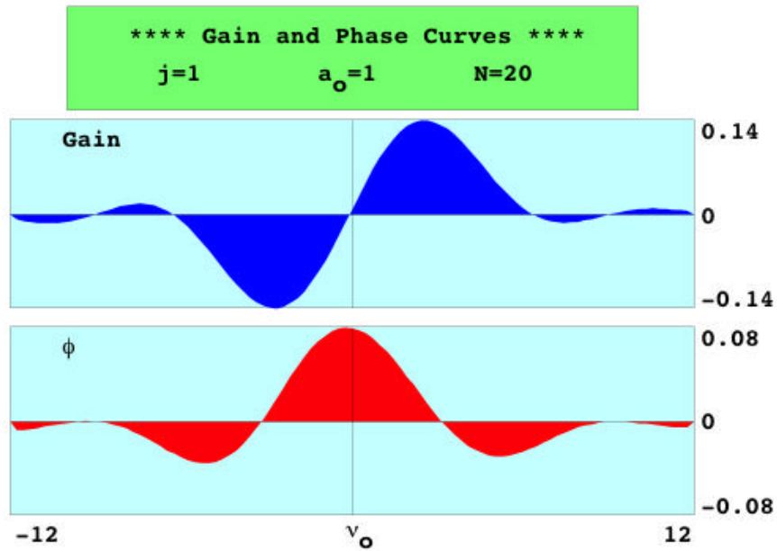
Figure 26. Weak field FEL gain and phase spectra
