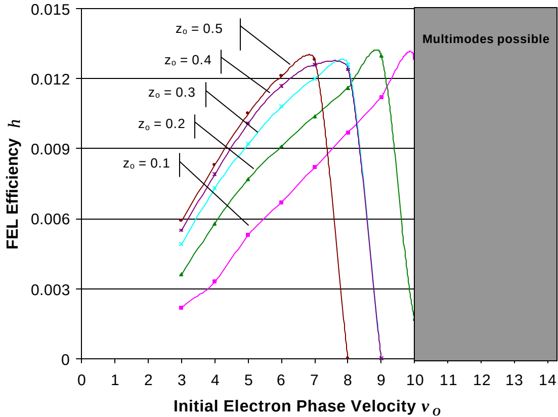
Figure 34. Strong Field Efficiency Simulation Results
