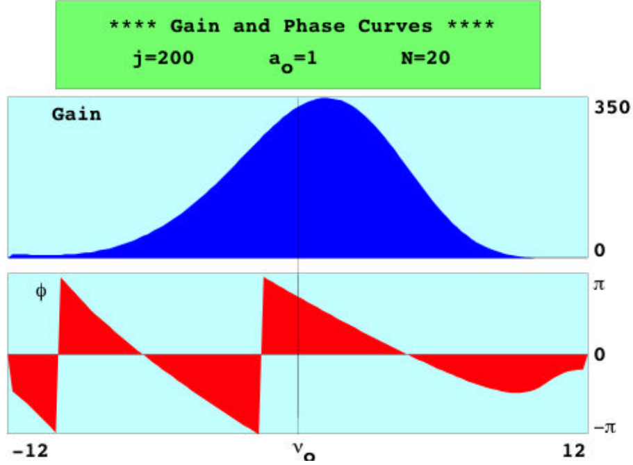
Figure 28. High current FEL gain and phase spectra
