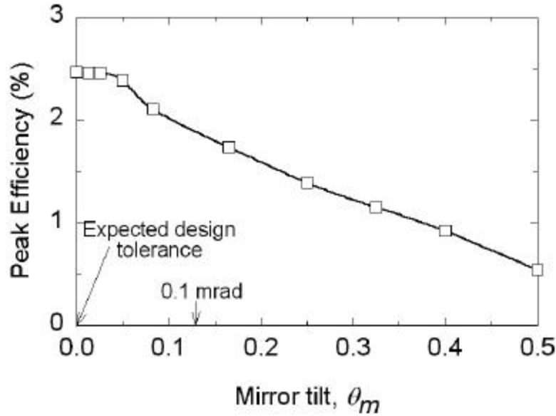
Figure 40. 1 MW Efficiency vs. Mirror Tilt
