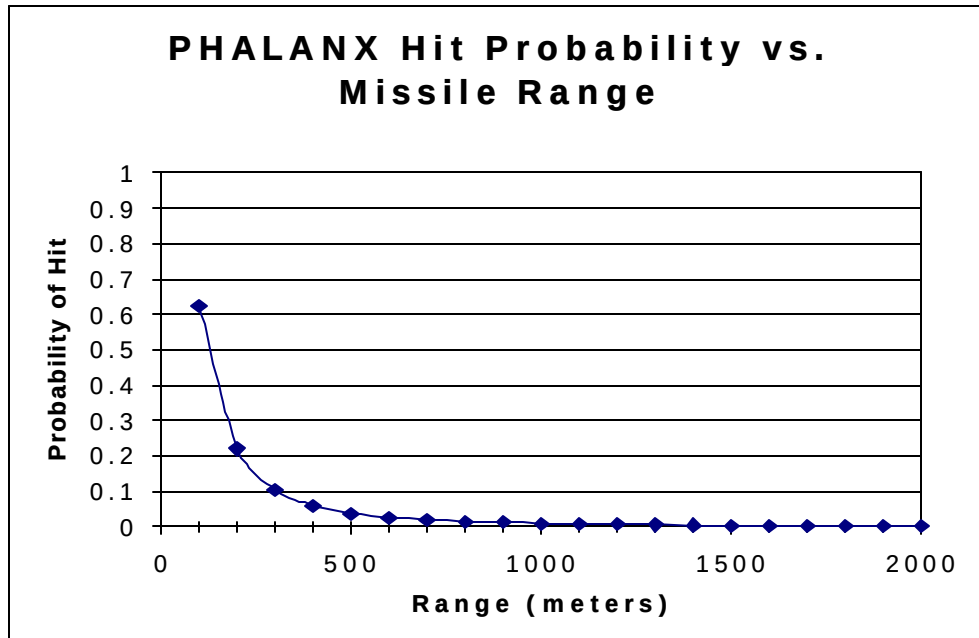
Figure 8. PHALANX hit probability
