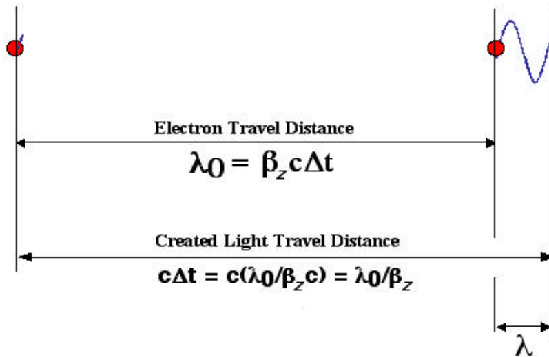
Figure 22. The Electron-Photon Race
