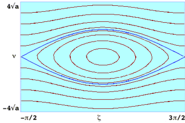
Figure 23. FEL open and closed orbits plotted in phase space
