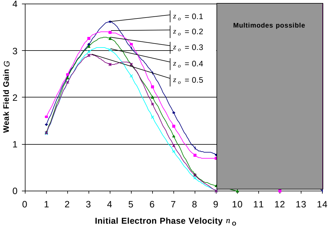
Figure 33. Weak Field Gain Simulation Results
