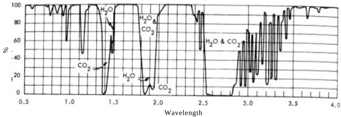
Figure 14. Transmittance of 1000 ft horizontal air path at sea level containing 5.7 mm precipitable water at 79° F
