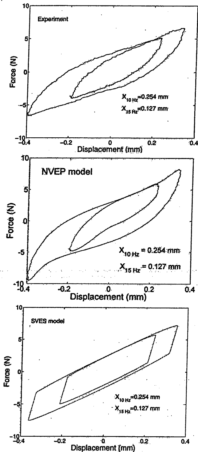
Figure 11. Dual frequency validation of SVES and NVEP hysteresis models for the preloaded MR On case for a 10 Hz amplitude of 0.254 mm and a 15 Hz amplitude of 0.127 mm.
