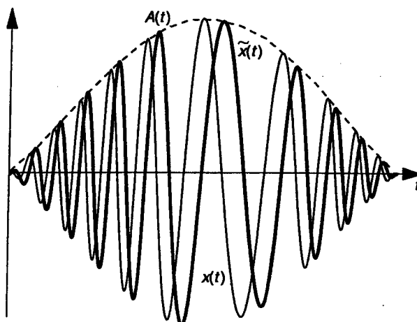
Figure 1 Real signal x(t) , Hilbert transform \tilde{x}(t) , and the signal envelope A(t) .
