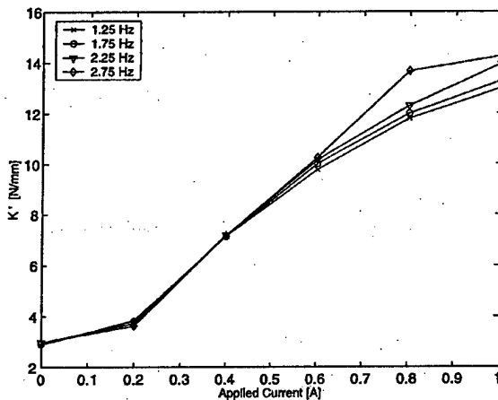
Fig. 4a Storage stiffness K' vs applied current.
