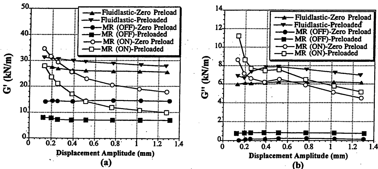
Fig. 7. Linearized constants obtained from the damper pair characterization: (a) stiffness modulus, G' , and (b) damping modulus, G'' .
