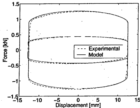
a) Bingham plastic force vs displacement
