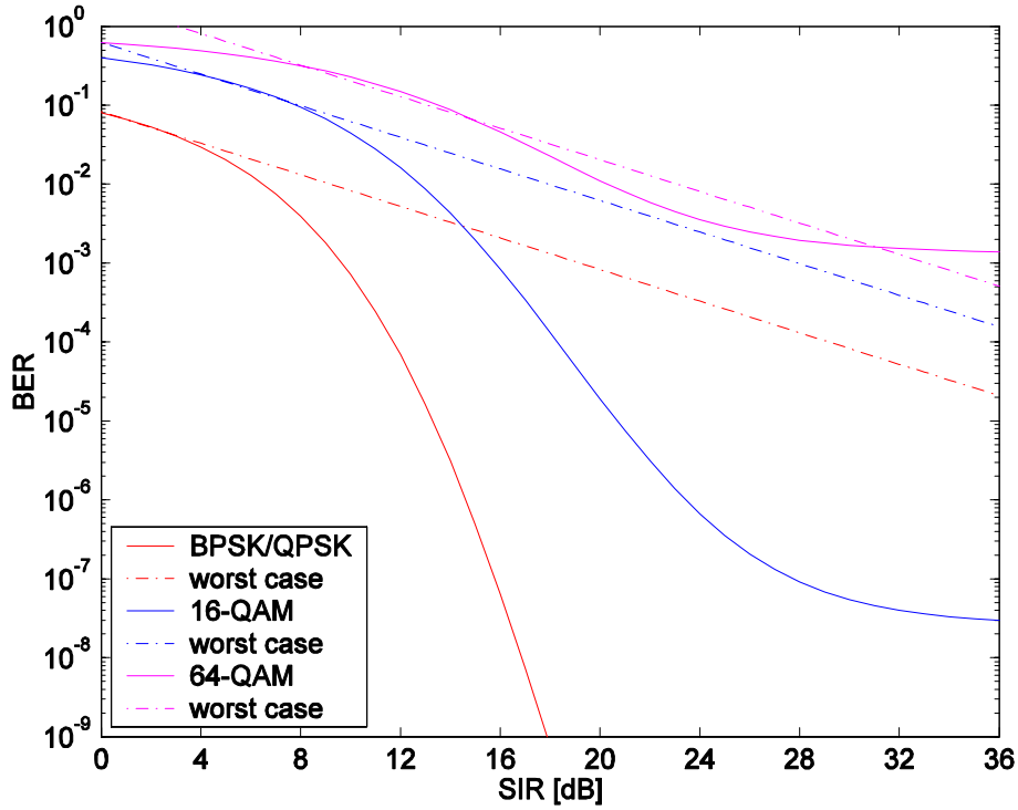
Figure 14. Performance of BPSK/QPSK, 16QAM and 64-QAM in AWGN with pulsed-noise jamming.
