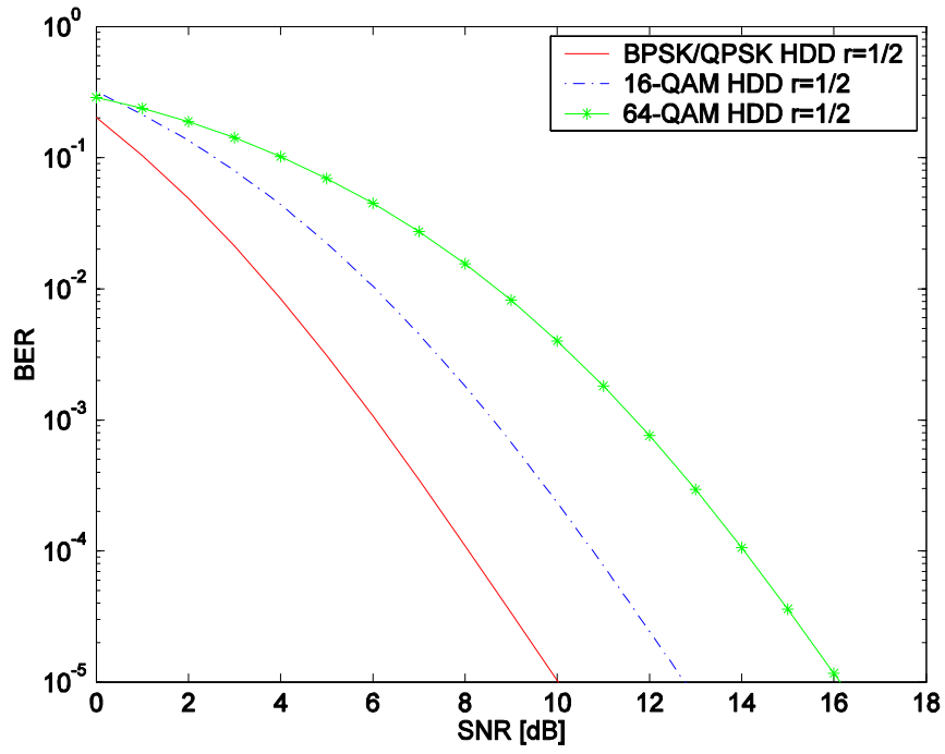
Figure 28. Performance of BPSK/QPSK, 16QAM and 16QAM with HDD ( r = 1/2 ) in Nakagami fading.
