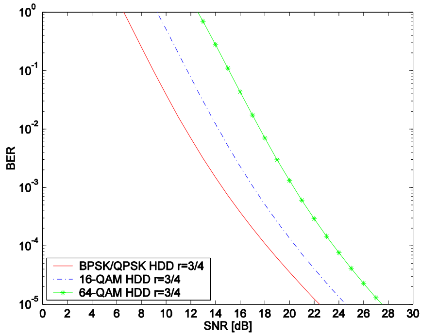
Figure 29. Performance of BPSK/QPSK, 16QAM and 16QAM with HDD ( r = 3/4 ) in Nakagami fading.
