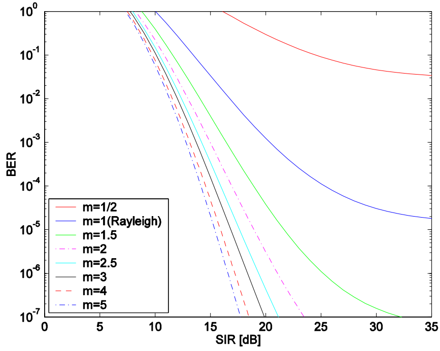
Figure 42. Performance of 16QAM with HDD ( r = 3/4 ) over Nakagami fading in pulsed-noise jamming, SNR = 24.5 dB and \rho = 0.5 .
