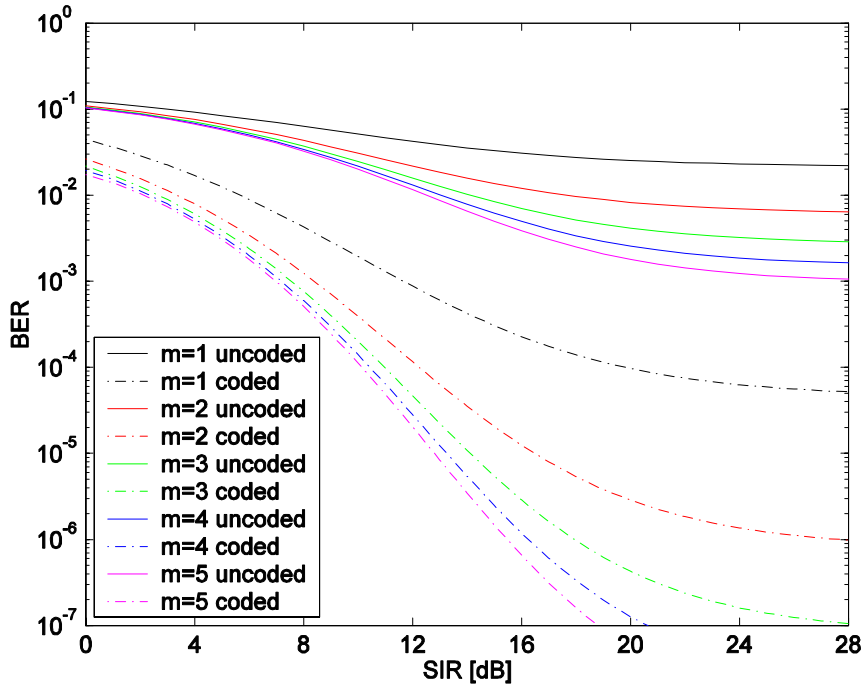
Figure 40. Uncoded vs. HDD( r = 1/2 ) 16QAM over Nakagami fading with pulsed-noise jamming where SNR = 13 dB and \rho = 0.5 .
