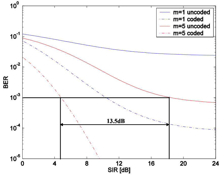
Figure 33. Range of coding gain for HDD BPSK/QPSK. ( r = 1/2 )
