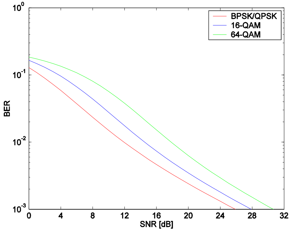
Figure 15. Performance of BPSK/QPSK, 16QAM and 16QAM in Nakagami fading.
