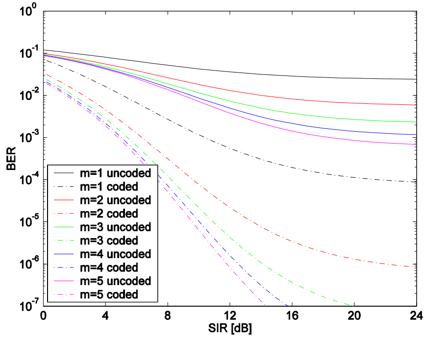
Figure 32. Uncoded versus HDD ( r = 1/2 ) BPSK/QPSK over Nakagami fading with pulsed-noise jamming where SNR = 10 dB and \rho = 0.5 .
