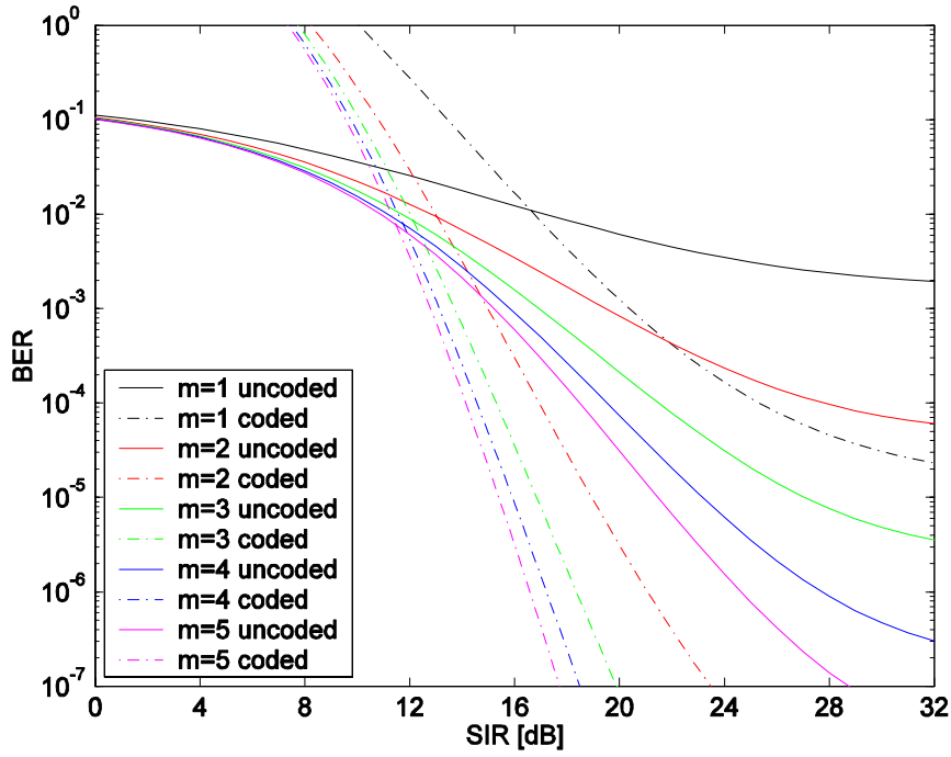
Figure 43. Uncoded vs. HDD ( r = 3/4 ) 16QAM over Nakagami fading with pulsed-noise jamming, SNR = 24.5 dB and \rho = 0.5 .
