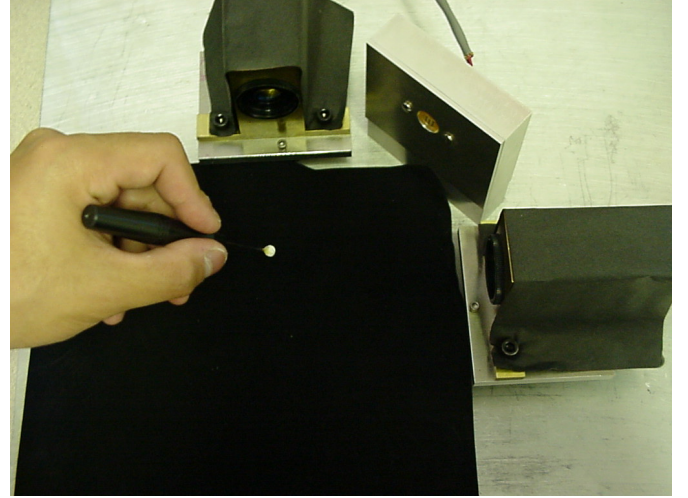
Figure 1. The ASAP system. The apparatus performs 3-D optical tracking of the white ball affixed to the tool tip.
