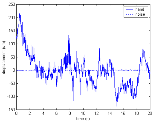
Figure 5. Sample data recorded from subject attempting to hold an instrument motionless in the Z axis. The dotted line represents a sample of the noise of the system.
