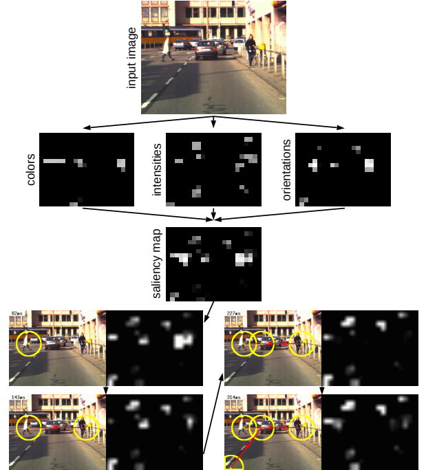
Fig. 1. Overview of the bottom-up attention front-end [5].
