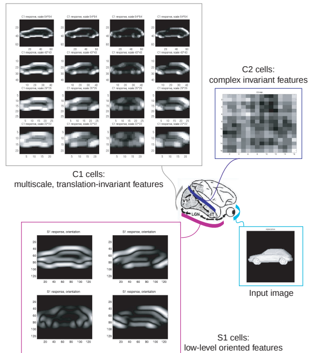
Fig. 2. The HMAX architecture for object recognition [9].
