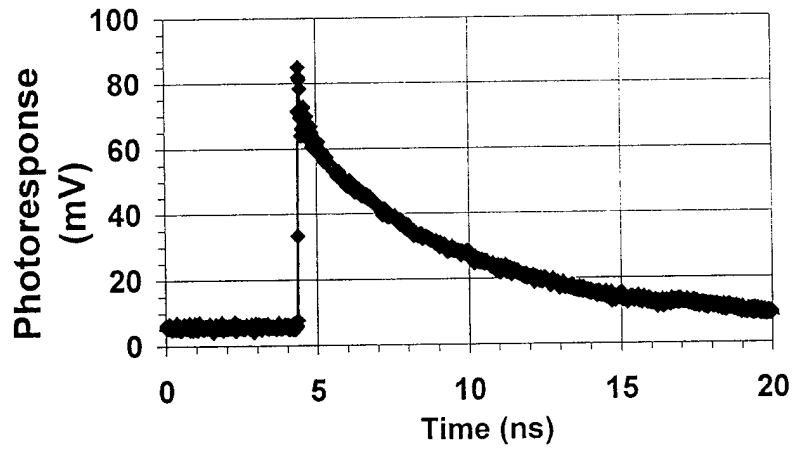
Photoresponse vs. Time T=85K, Ib=40mA Sample ATL1I(a)
