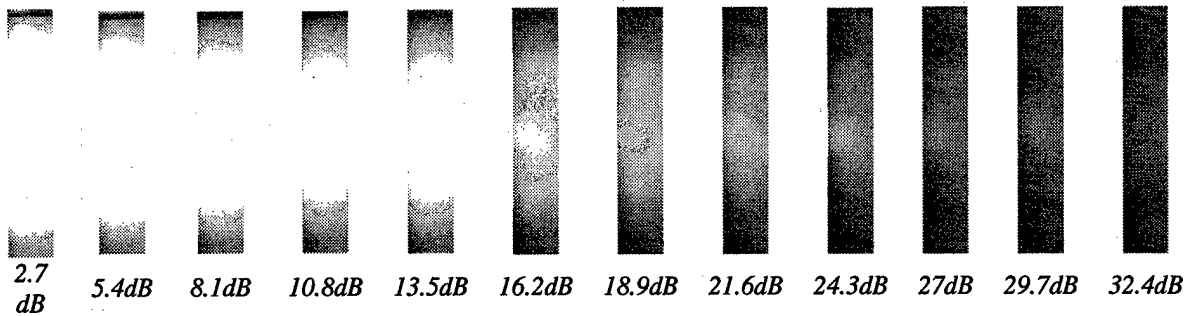
Figure 2. Twelve steps of the dynamic range phantom with associated attenuation @ 3.85 MHz.
