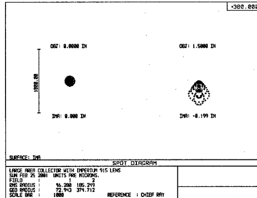
Figure 9b 3-in. Lens with 375 micron spot size
