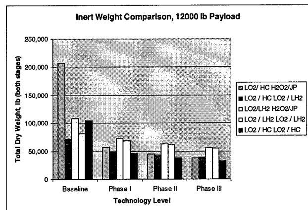
Figure 5. Inert Weight Comparison
