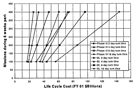
Figure 11. Mission Capability vs. LCC
