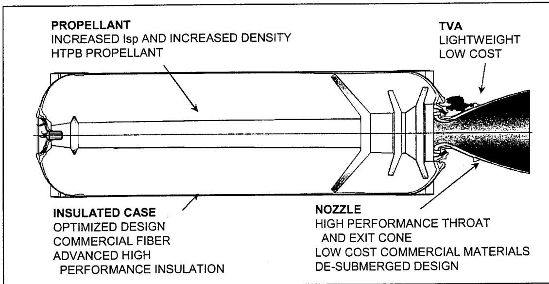
Figure 8. Phase I Solid Boost Demonstrator
