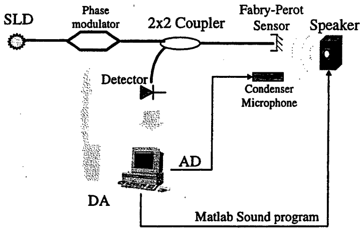
Figure1 Fabry-Perot sensor system
