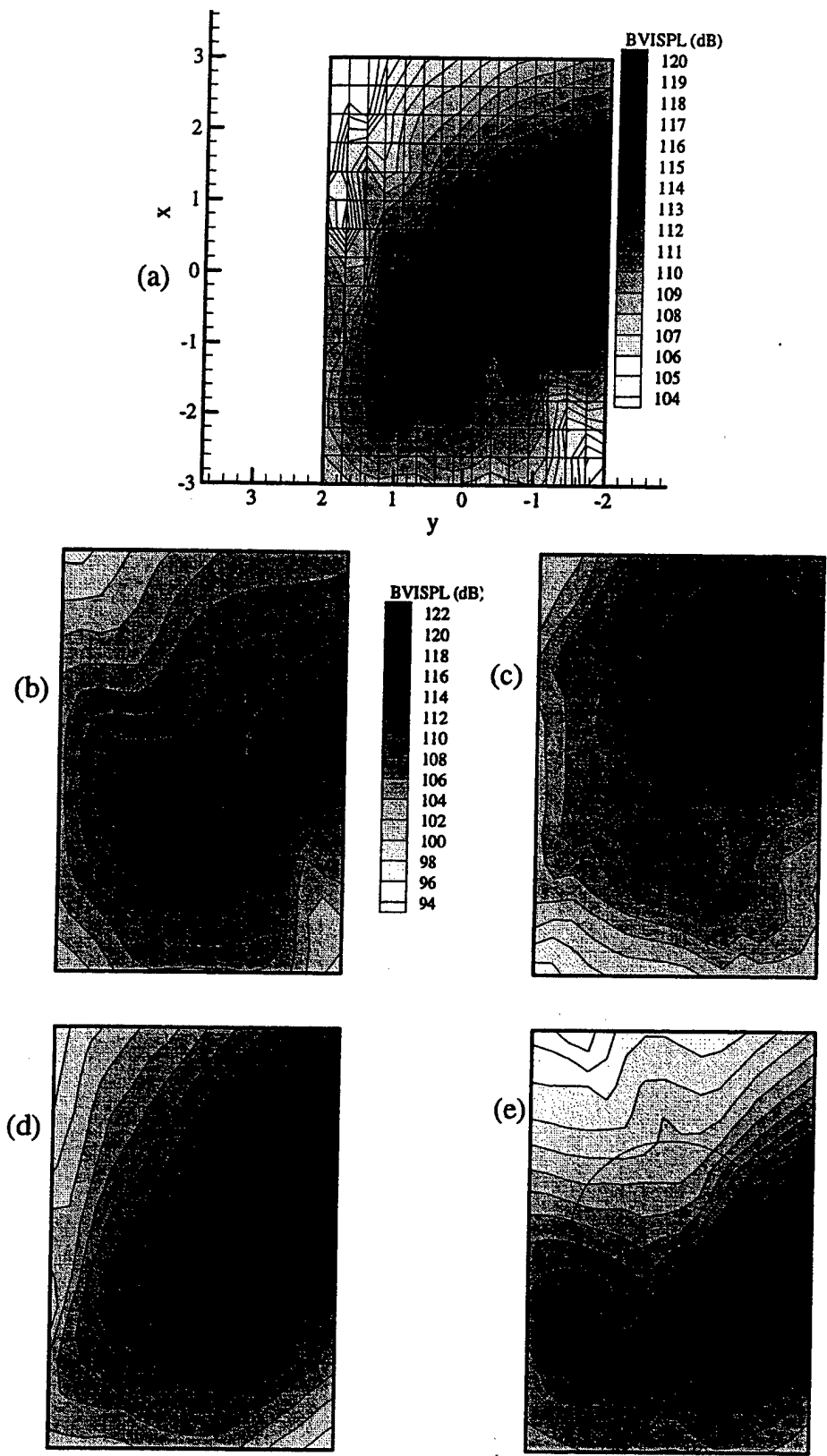
Figure 4: Noise (BVISPL) generated by the loading from (a) all the tip vortices (entire wake) (b) tip vortex from reference blade, k-0, (c) tip vortex from previous blade, k-1, (d) tip vortex from opposite blade, k-2, and (e) tip vortex from k-3.
