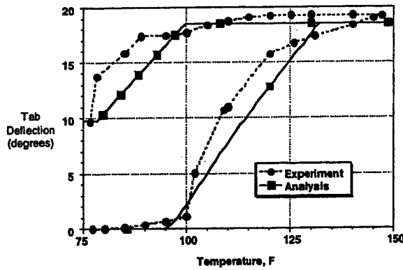
Figure 3: Benchtop testing
