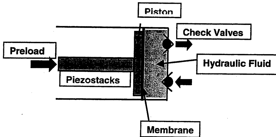
Figure 1 Schematic of piezostack driven hydraulic pump
