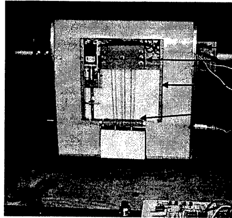
Blade Tab Actuated with Shape Memory Alloys Actuator, Wing Section Tested in Open-Jet Wing Tunnel; Produced Tab Deflections of over 20 deg.
