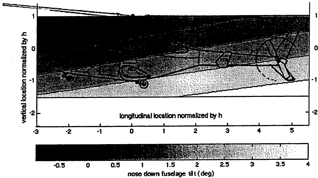
Figure 1: Fuselage tilt (degrees, nose down) as a function of added drag device location (non-dimensionalized by the distance h between hub and center of gravity, measured along shaft axis). This figure corresponds to a Bell 222B helicopter, which is inscribed in the contour plots to scale. For a given fuselage location of an added drag device generating a drag force equal to 5% of helicopter weight, the contours indicate the resulting nose-down fuselage tilt in degrees for the above descent flight conditions. Notice that fuselage tilt due to added drag depends much more strongly on the vertical location of the drag device than on its longitudinal location; the opposite is observed for the case of added lift, which generates a fuselage tilt of comparable magnitude but a much smaller change in TPP angle.
