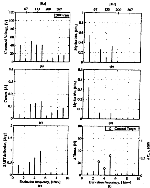
Figure 4 Closed loop test, control parameter thrust: simultaneous control targets 22, 11 and 32 N at 3, 4 and 5/rev; hover, 2000 rpm, 2 deg collective
