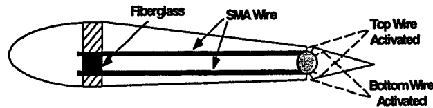
Figure 1: Tab actuation mechanism
