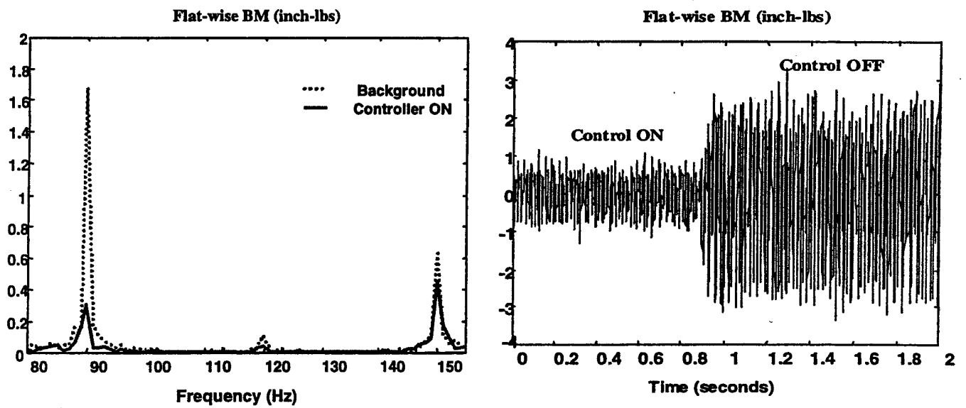
Figure 5: Single load case (blade root flat-wise bending moment control, 1800 RPM, 0.3 advance ratio, 6 deg collective pitch)
