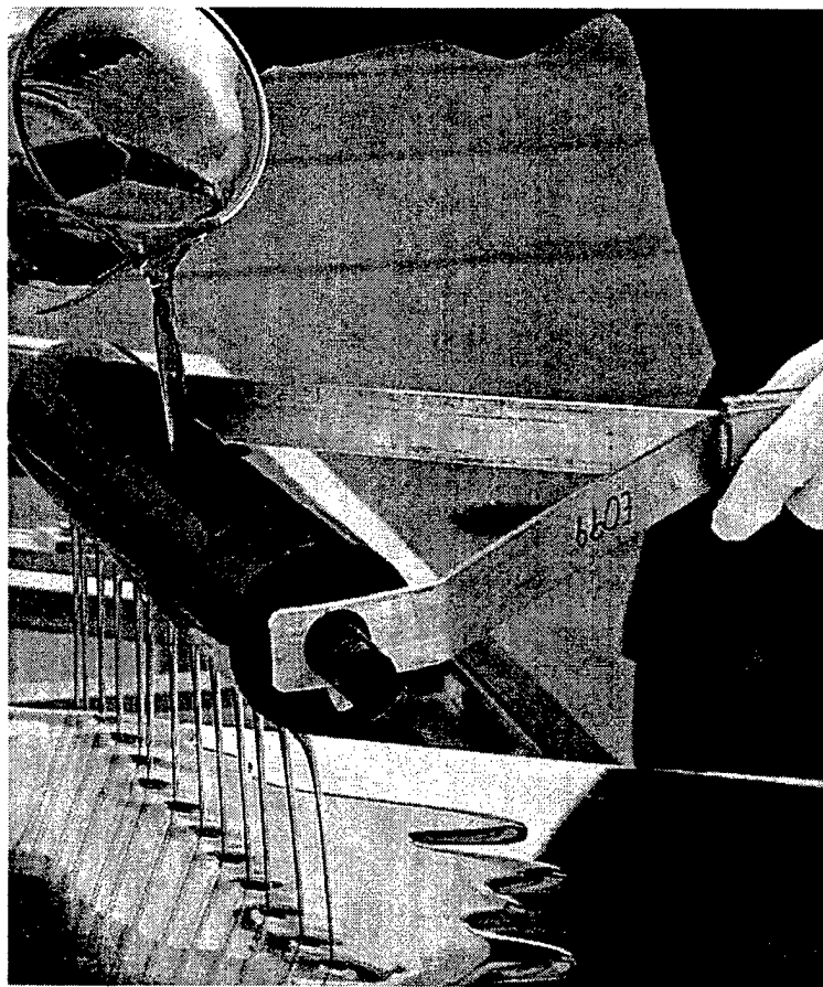
FIGURE 6. FLUID APPLICATION AND SPREADER
