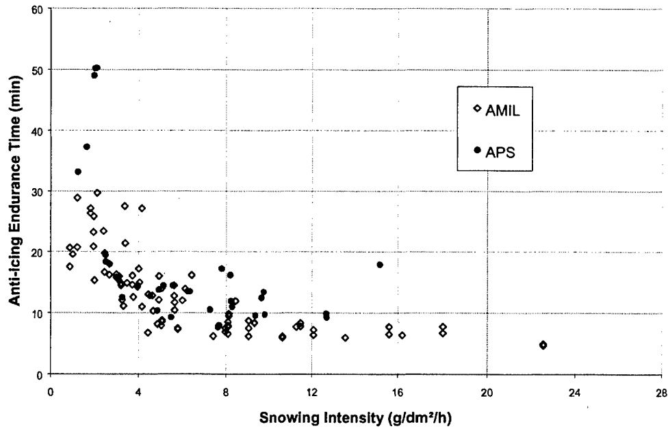
FIGURE 16. OUTDOOR SNOW TESTS AT TEMPERATURES RANGING FROM -3° TO -10°C
