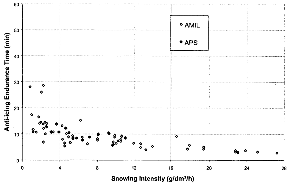
FIGURE 17. OUTDOOR SNOW TESTS AT TEMPERATURES RANGING FROM -10° TO -25°C
